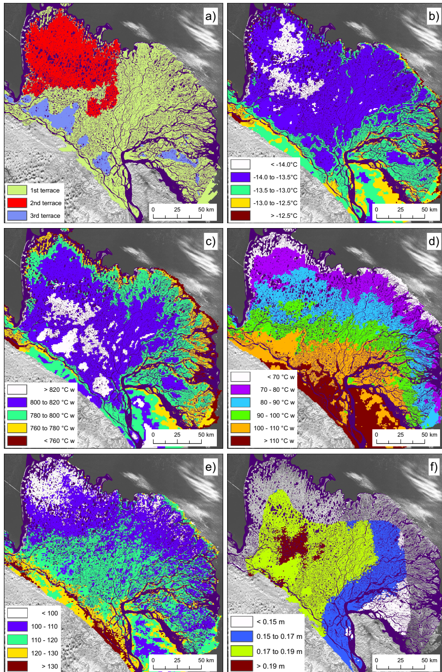
Figure 5. Spatial distribution of model input data sets in the LRD (Sects. 3.2, 3.3): a) subsurface classification (compare Table 1); b) average surface temperature 2004-2013; c) average freezing degree weeks 2004-2013; d) average thawing degree weeks 2004-2013; e) average number of snow-free days 2004-2013; f) average snow depth 2004-2013 for a snow density of 225\text{kg m}^{-3} .
