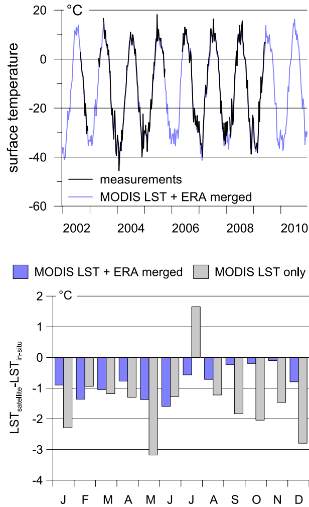
Figure 2. Top: daily average surface temperatures measured on Samoylov Island (Langer et al., 2013; Boike et al., 2013) vs. surface temperatures synthesized from MODIS LST and ERA reanalysis. Bottom: difference between satellite-derived LST and in-situ measurements for monthly averages of periods when in-situ measurements are available (see top figure). See text.
