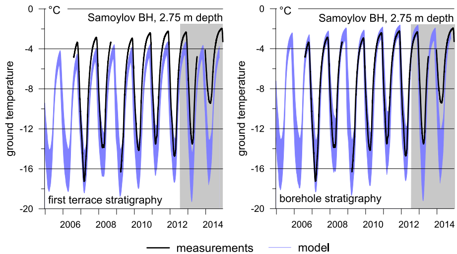
Figure 8. Modeled and measured ground temperatures for the borehole on Samoylov Island. Left: subsurface stratigraphy of the first terrace (Table 1). Right: stratigraphy adapted to the true ground conditions at the borehole (0-0.5 m: 30% water/ice, 10% air, 60% mineral, sand; 0.5-9 m: 40% water/ice, 60% mineral, sand; deeper layers as for first terrace, Sect. 4.2.1). The blue area depicts the spread between model runs with snow densities of 200 and 250 kg m -3 . Periods for which in-situ data are affected by new installations at the Samoylov station are marked in grey. These should not be used for comparison, see text.
