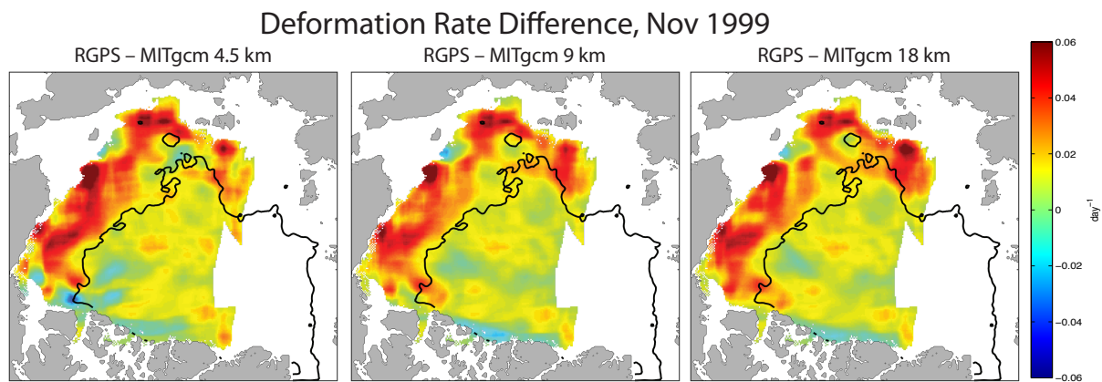
Figure 5. Smoothed (150 km) difference in deformation rate \dot{D} between RGPS and model solutions with 4.5 km 4.5 km (left), 9 km 9 km (middle), and 18 km 18 km (right) grid spacing. Largest differences occur in the seasonal ice zone outside the black contour.
