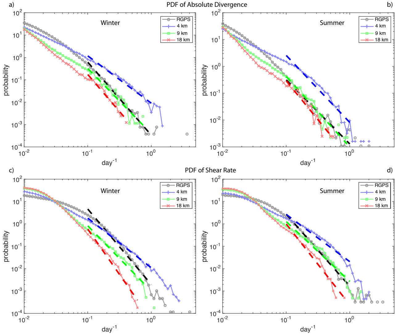
Figure 9. Probability density function of absolute sea-ice divergence |\dot{\nabla}| (a, b) and shear rate \dot{\tau} (c, d) for a length scale of 20 km based on 5-daily aggregated Lagrangian cells for all winter (Nov–Apr) and summer (May–Aug) periods for RGPS and model solutions. Dashed lines are least square fits to the approximately linear part of the PDFs between 0.05 and 1.0 \text{day}^{-1} . Note the logarithmic axes scaling.
