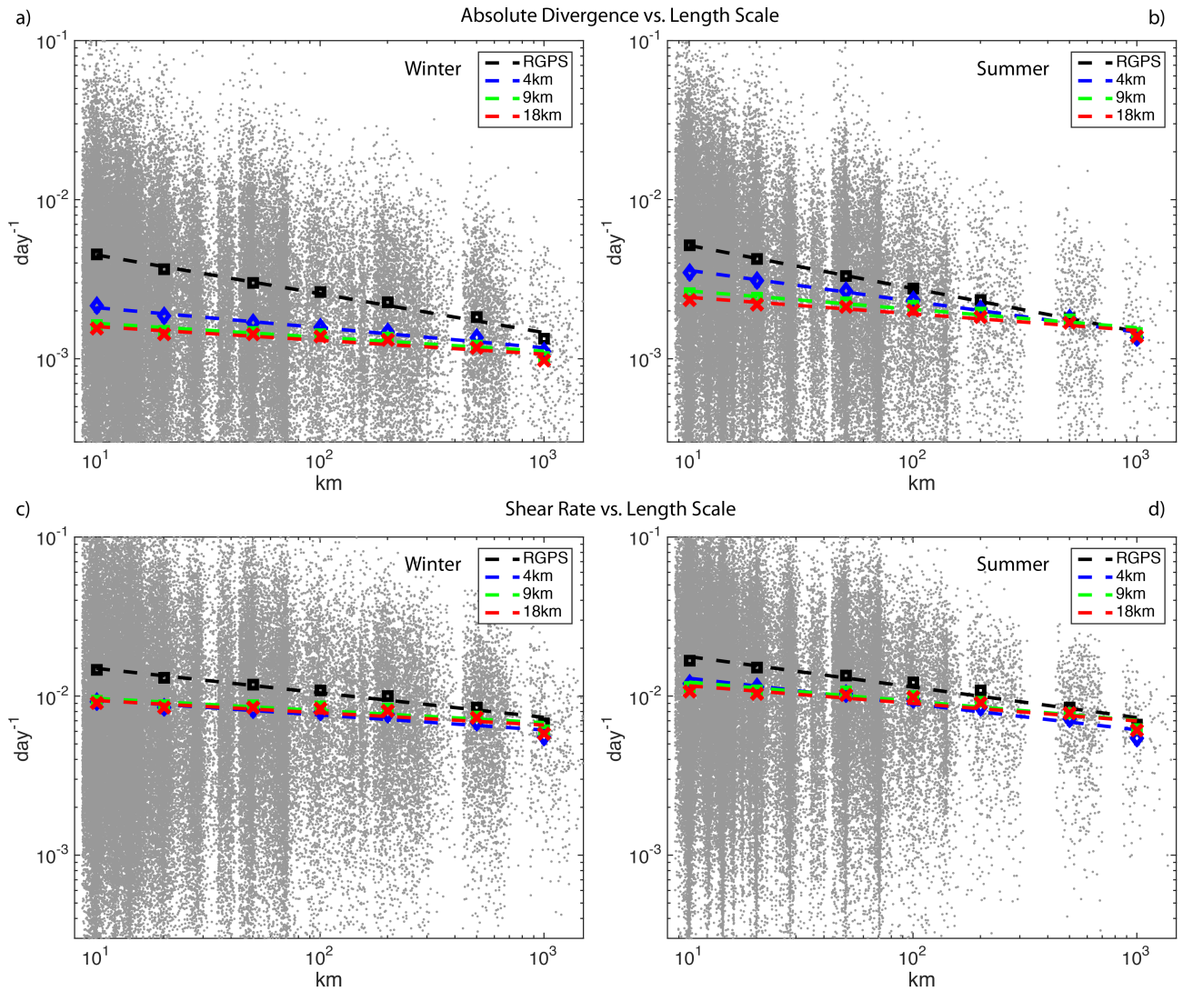
Figure 8. Scaling properties of absolute sea-ice divergence |\nabla\vec{v}| (a, b) and shear rate \dot{\gamma} (c, d) for RGPS and model solutions for all winter (Nov–Apr; Nov–May; a, c) and summer (May–Jun; May–Aug; b, d) periods. For length scales of 10, 20, 50, 100, 200, 500, and 1000 km the ice divergence and shear from the Lagrangian cells were aggregated over 5-day periods. Individual data points for the RGPS dataset are shown in grey. Mean values for the six different length scales are marked with symbols. Dashed lines are least square fits to the six mean values from 10 to 1000 km. Note the logarithmic axes scaling.
