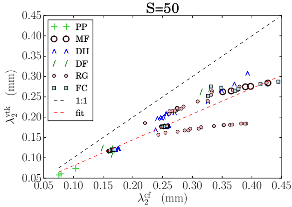
Figure 2. Comparison between smoothing parameter S = 50 (left) and S = 200 (right) for the top. Top : Representation of the triangulated surface of a subsection of a snow sample. In the middle : Scatter plots of the Porod length \lambda_1^{cf} versus \lambda_1^{v tk} , including a fit (red dotted line). At the bottom : Scatter plots of the curvature-length \lambda_2^{cf} versus \lambda_2^{v tk} , including a fit (red dotted line).
