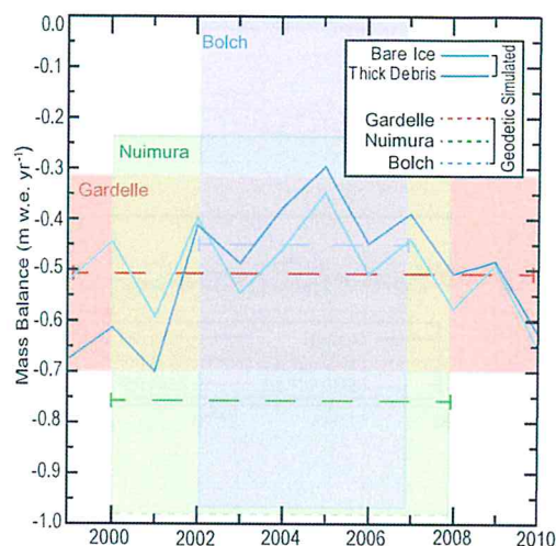
Figure 7: Simulated mass balance during the 1999-2010 calibration period, for the two model configurations. The dashed red line represents the geodetic mass balance from Gardelle et al. (2013), to which the model is calibrated from 1999-2010. Also included are the geodetic mass balance surveys of Bolch et al. (2011) and Nuimura et al. (2012), with the width of the lines representing the duration of study. Coloured boxes represent the uncertainty associated with each survey. Nuimura et al. (2012) lower bound of uncertainty is curtailed.
