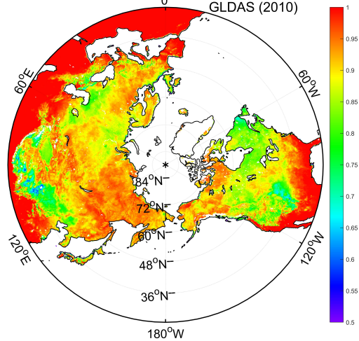
Comparison of FT map(A) and modelled soil temperature GLDAS (2010)
