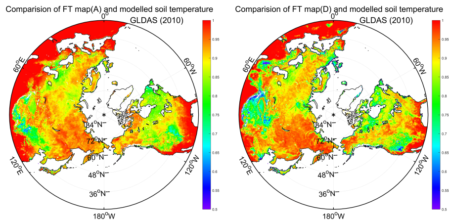
Fig. 1. Comparison of F/T map with soil temperature modelled by GLDAS
