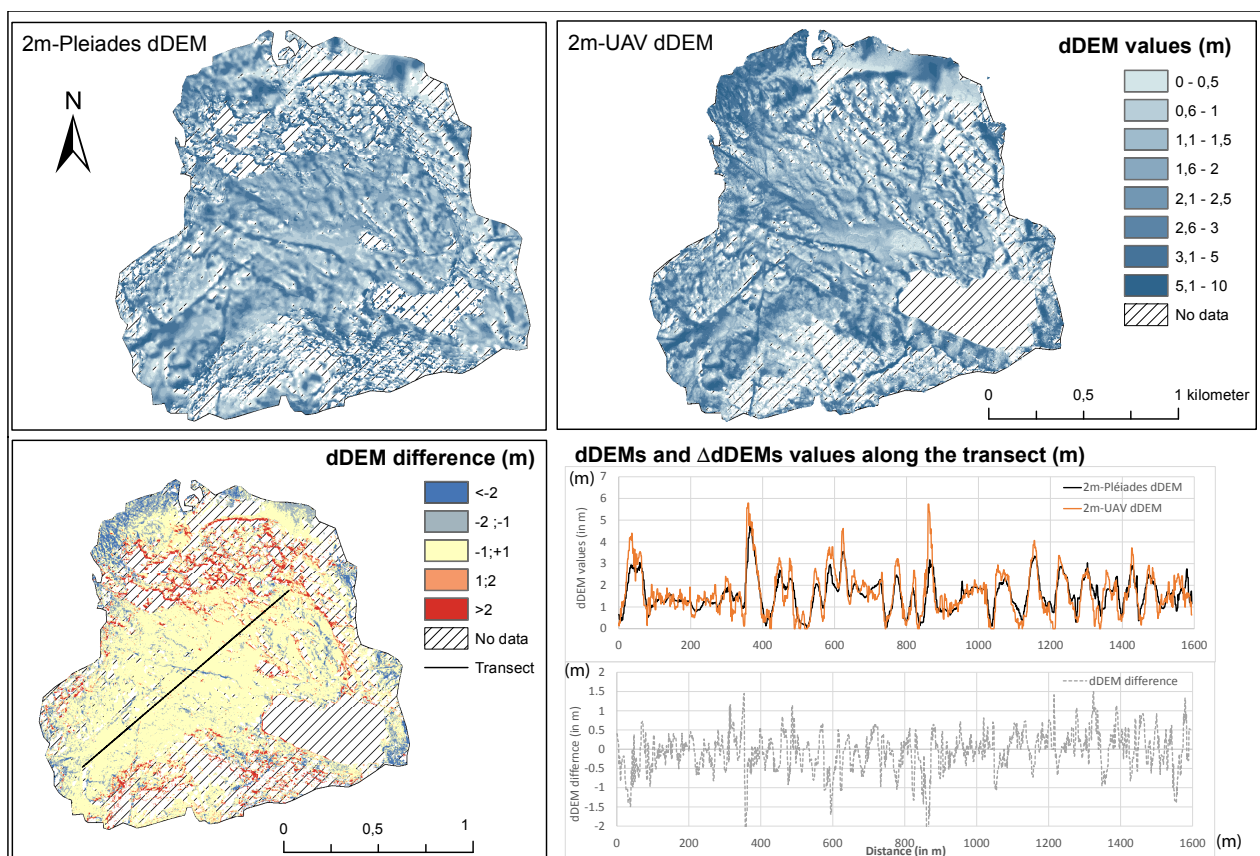
Figure 9. Pléiades and UAV dDEM, and dDEM differences. dDEMs and \Delta dDEMs (dDEMs differencing) values along the transect.
