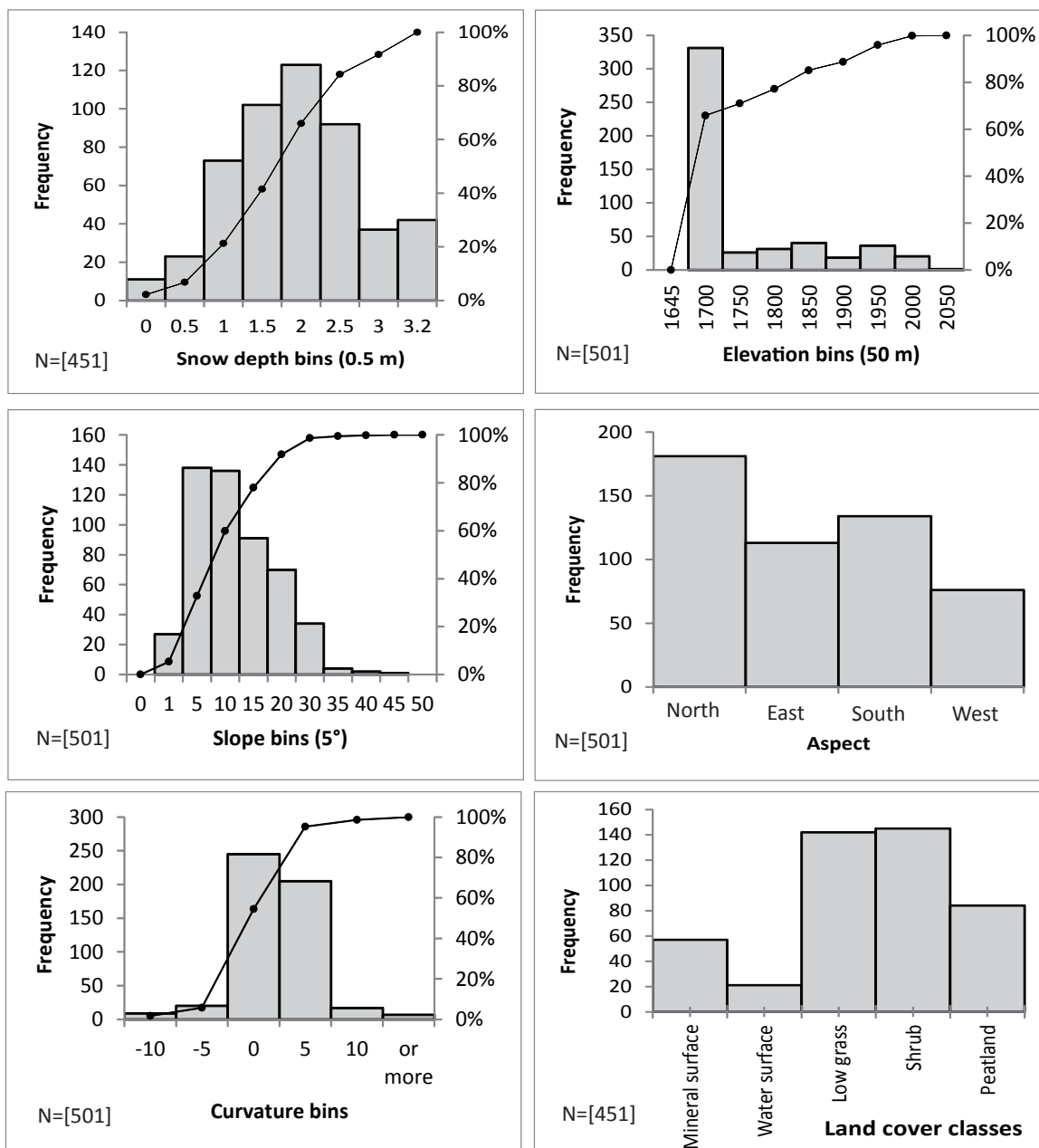
Figure 3. Distribution of the snow probe sampling, according to the snow depth, the elevation, the slope, the aspect, the curvature and the land cover classes. On the whole snow probe sampling (N=501), the snow probe did not reach the ground for 50 occurrences.
