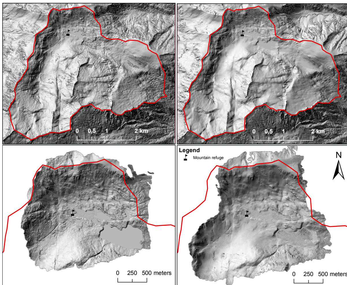
Figure 5. Hillshade of snow free 2 m-Pléiades (top-left) and 1 m-UAV DEM (bottom-left) DEMs, and winter 2 m-Pléiades (top-right) and 1 m-UAV (bottom-right) DEMs.
