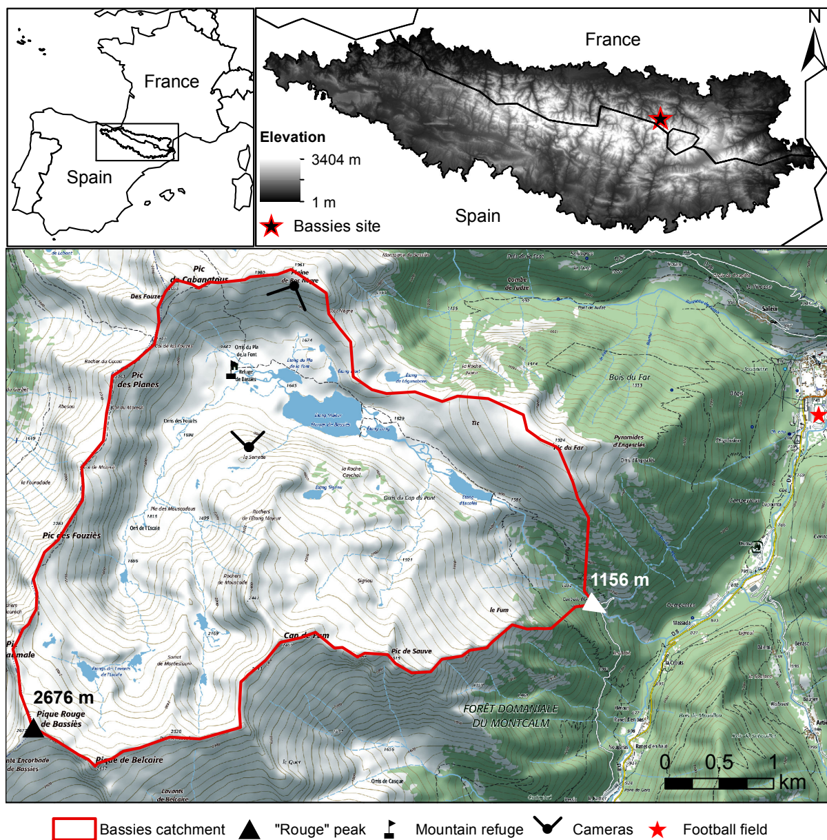
Figure 1. Top: localization of study site relative to Europe, and to the Pyrenees mountain. Bottom: Bassies catchment (14.5 km 2 ) on a Top 25 topographic map from ©IGN (“Institut national de l’information géographique et forestière”) map.
