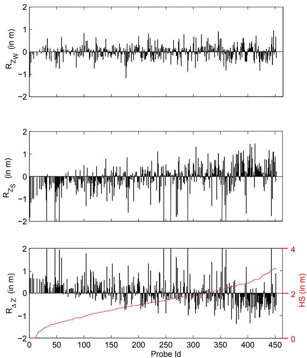
Figure 10. Residual error terms, after the systematic error removal, for the 2 m-Pléiades winter DEMs, the snow-free 2 m-Pléiades DEM, and the 2 m-Pléiades dDEM according to the probe Id ranked in the ascending HS order (see equation section 4).
