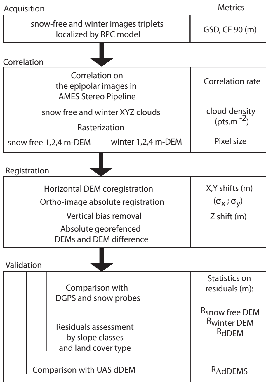
Figure 4. Successive phases in Pléiades triplets processing, and associated metrics of assessment.
