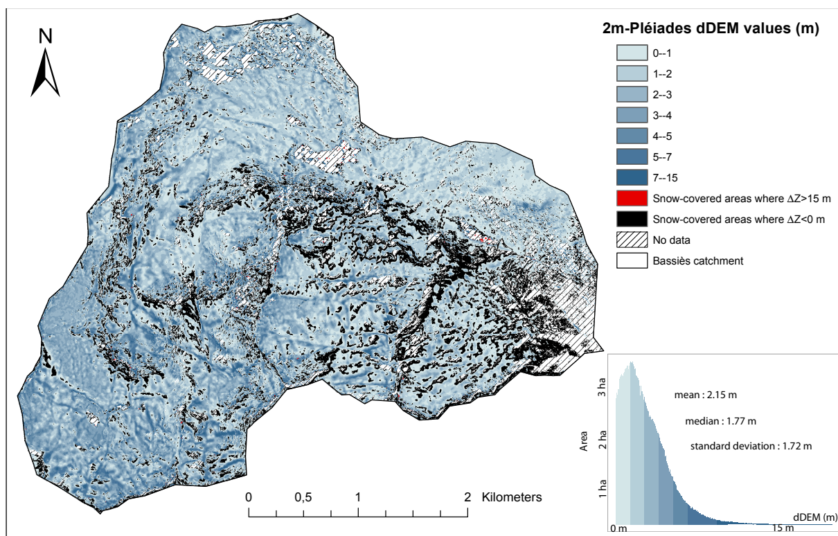
Figure 6. 2 m-Pléiades dDEM map interpreted as snow height ( m) in Bassiès catchment.
