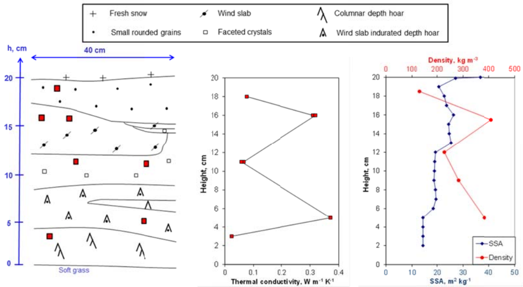
720 Figure 7. Stratigraphy and vertical profiles of snow physical properties near our study site on 14 May 2014. Fresh snow is just a 2 mm-thick sprinkling, also visible in the SSA profile. Density data are for the middle of the 3 cm-high sample. Snow type symbols are those of (Fierz et al., 2009), except for the lower wind slab which transformed into depth hoar to form an indurated layer, as detailed in the text. Red-filled black squares in the stratigraphy indicate where thermal conductivity measurements were made.
