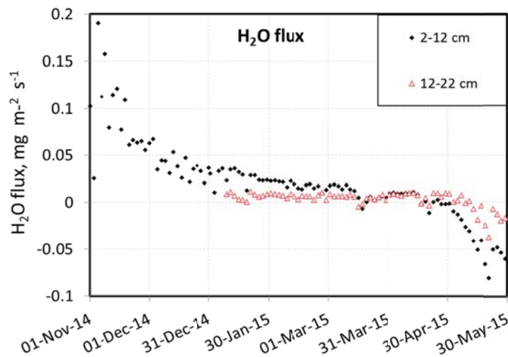
750 Figure 12. Time series of the water vapor flux at two levels in the snowpack. Positive fluxes are upward.
