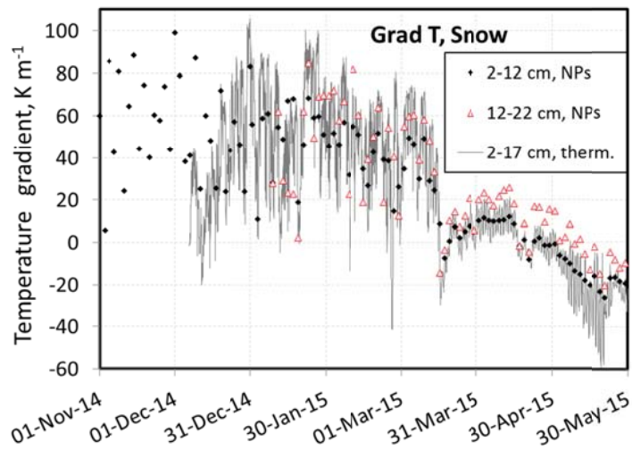
745 Figure 11. Time series of the temperature gradient in the snow. Values were obtained from the heated needle probes at 2, 12 and 22 cm, with a data point every 2 days. Thermistors at 2 and 17 cm also measured temperature every hour, and the values are shown with an hourly resolution. The different start dates of each curve are determined by the date where the snow height reached the relevant level.
