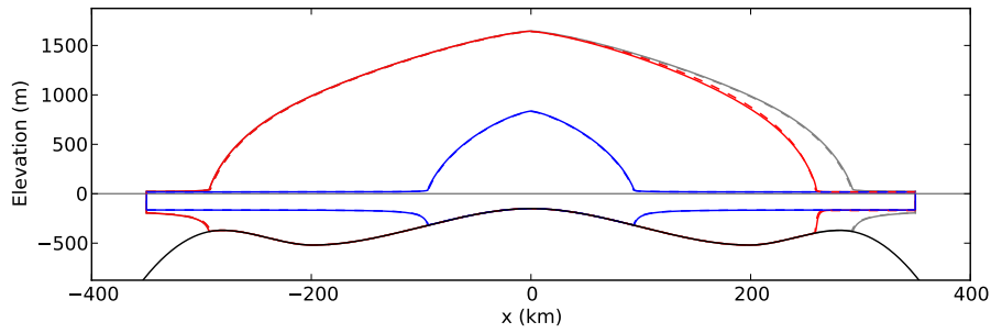
Figure 2. Ice sheet profiles at three different stages of the flow-line simulations 2D_{\alpha=\frac{1}{2},\beta=\frac{1}{2},\gamma=1} (continuous) and 2D_{\text{ref}} (dashed). Output of the reference simulation is scaled by factor 0.5 in both horizontal and vertical direction to allow for comparison of shapes between the two simulations.
