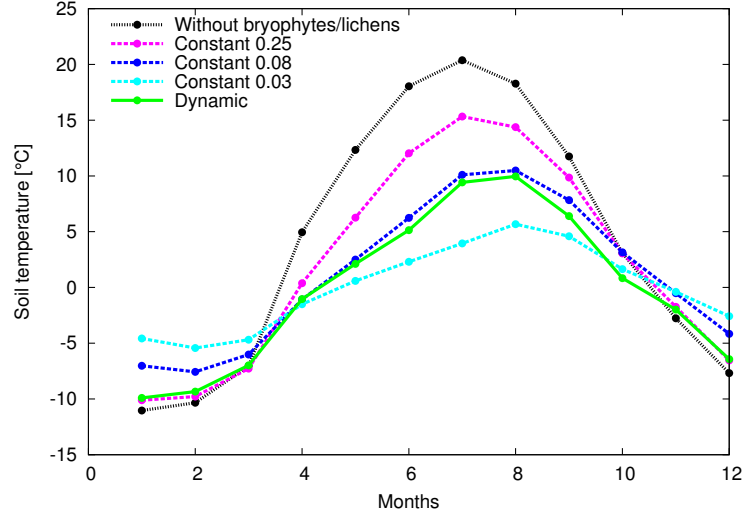
Figure 7. Temperature of the uppermost soil layer of a model grid cell at 55° 30' N, 98° 30' W, which is also used for the sensitivity analysis (Sect. A in the appendix). The dots stand for monthly average values for the period 1996 to 2010. “Without” denotes a transient simulation from 1901 to 2010 without a bryophyte and lichen layer. “Constant 0.25” denotes an equivalent simulation, but including an organic layer with constant coverage and thermal properties. The thermal conductivity of this layer is set to 0.25 [W K -1 m -1 ] as in Ekici et al. (2014). “Constant 0.08” corresponds to an organic layer calibrated to reproduce topsoil temperature under the bryophyte and lichen layer in summer. “Constant 0.03” corresponds to an organic layer calibrated to reproduce average annual topsoil temperature under the bryophyte and lichen layer. “Dynamic” stands for a bryophyte and lichen layer with dynamic coverage and thermal properties.
