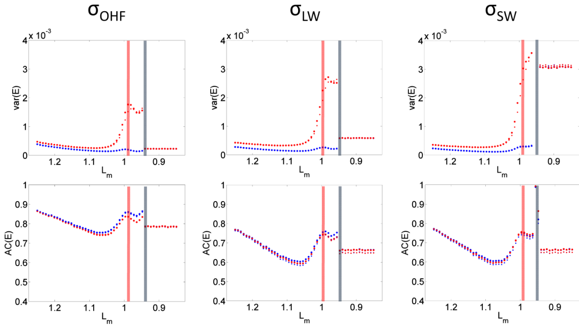
Figure 4. Variance (var) and autocorrelation (AC) of state E as a function of long-wave balance L_m in the model E12 with large red noise. In each column, the noise term has been introduced to one of three different terms, namely the ocean heat flux (OHF), long-wave radiative balance (LW) and short-wave radiative balance (SW). Winter sea ice is shown in blue, summer sea ice in red (seasons as in Fig. 1). The vertical shaded lines indicate the values of L_m where the annual minimum (red lines) and maximum (blue lines) ice volume reaches zero.
