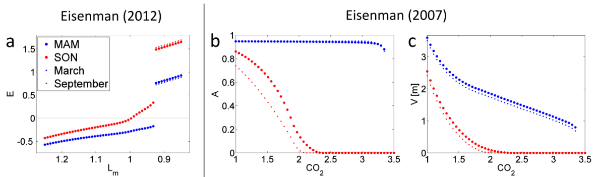
5 Figure 1. Response of the two column models to warming. a) Enthalpy versus surface longwave balance L_m in E12. The horizontal line demarcates between positive E (open water) and negative E (ice covered ocean). b) Ice-area fraction and c) ice volume (given as an equivalent thickness) versus CO_2 (given as multiples of the pre-industrial value) in E07. Each dot represents a time mean over the season indicated in the legend of subfigure (a).
