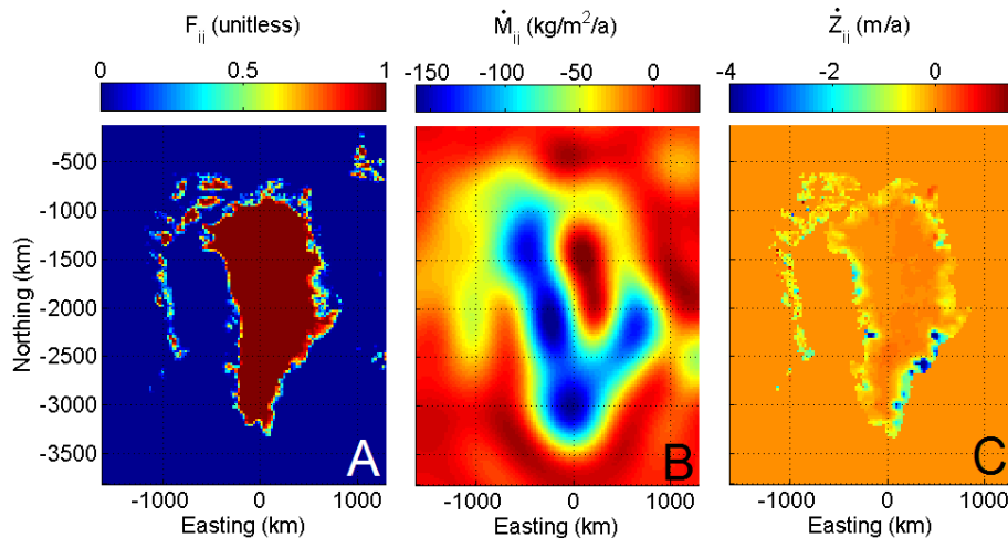
Fig. 1. Three independent pieces of information required as algorithm input. (A) Fractional ice coverage ( \bar{F} ), derived from glacier inventories generated by optical imagery (Arendt et al., 2012; Citterio and Ahlstrøm, 2013). (B) Spherical harmonic representation of cryosphere-attributed mass changes ( \dot{M}^G ), derived from gravimetry (Luthcke et al., 2013). (C) Ice surface elevation changes ( \dot{Z} ) derived from altimetry (Gardner et al., 2011; Schenk and Csatho, 2012). Map extent corresponds to inversion domain extent. Coordinates in polar stereographic projection.
