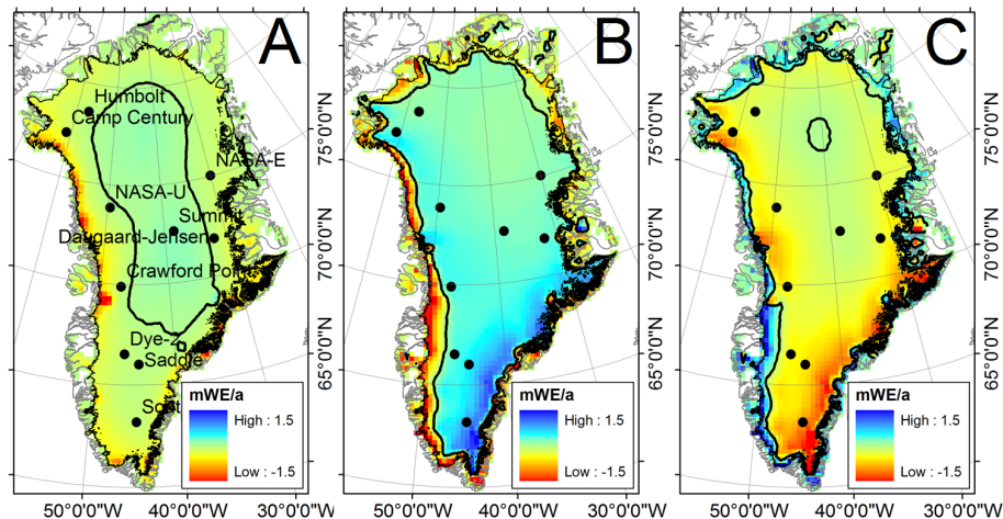
Fig. 9. IMBIE period (2004 to 2010) glacier continuity. (A) HIGA-inferred mass balance ( \dot{m} ; same as Fig. 6). (B) MAR modelled surface mass balance ( \hat{b} ). (C) Residual horizontal divergence of ice flux ( -\nabla Q ). The inverse \nabla Q field is shown to maintain a convention of blue shading for mass gain and red shading for mass loss. Black dots denote in situ measurements of Hamilton and Whillans (2002). Black contours denote 0 \text{ mWE a}^{-1} . All values given as per unit area .
