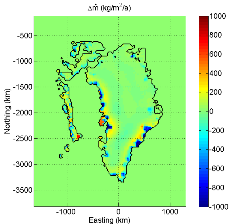
Fig. 5. Difference in specific mass balance ( \Delta \dot{m} ; e.g. per unit ice area ) of the HIGA product, which includes altimetry-derived information, relative to the strict gravimetry-inversion product of Colgan et al. (2013), which does not include altimetry information. Black lines denote the extent of ice-containing nodes within the Canadian Arctic and Greenland. Coordinates in polar stereographic projection.
