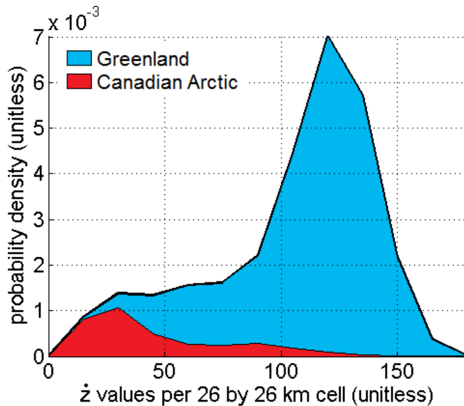
Fig. 2. Probability density functions of the altimetry-derived ice surface elevation change rates ( \dot{z} , at 2 km resolution) observed per 26 by 26 km grid cell in both Greenland and the Canadian Arctic.
