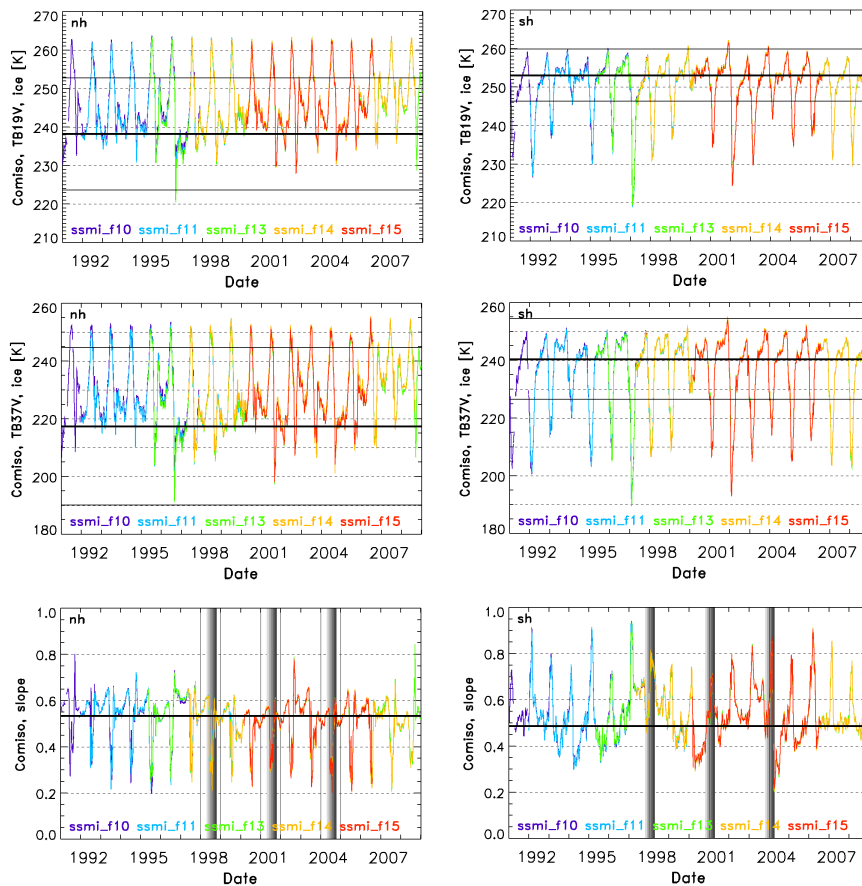
Fig. 1. Bootstrap F tie-points
