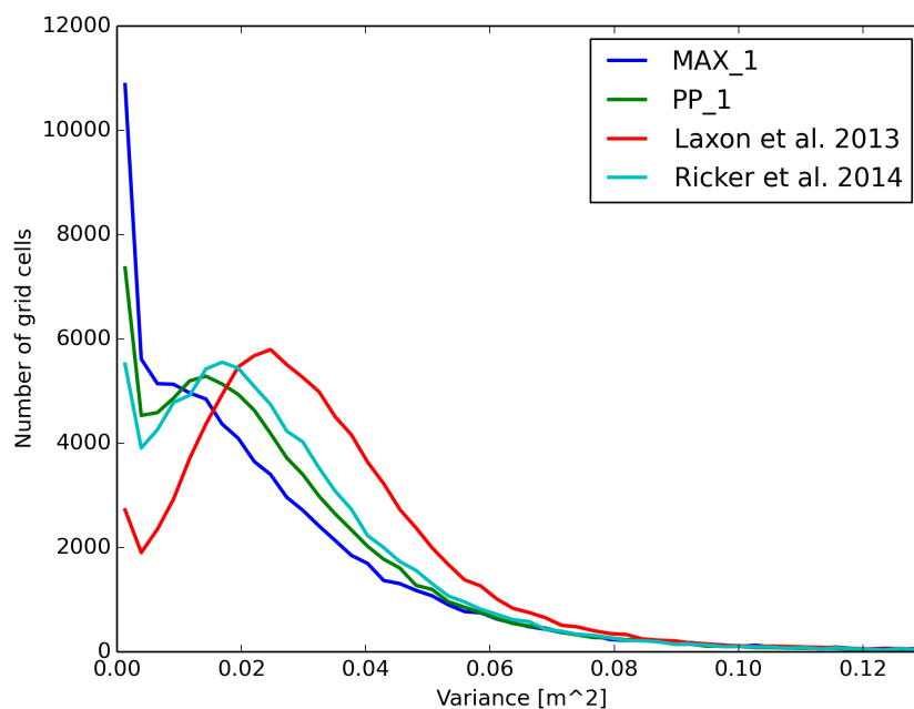
Fig. 1. Variance distribution
