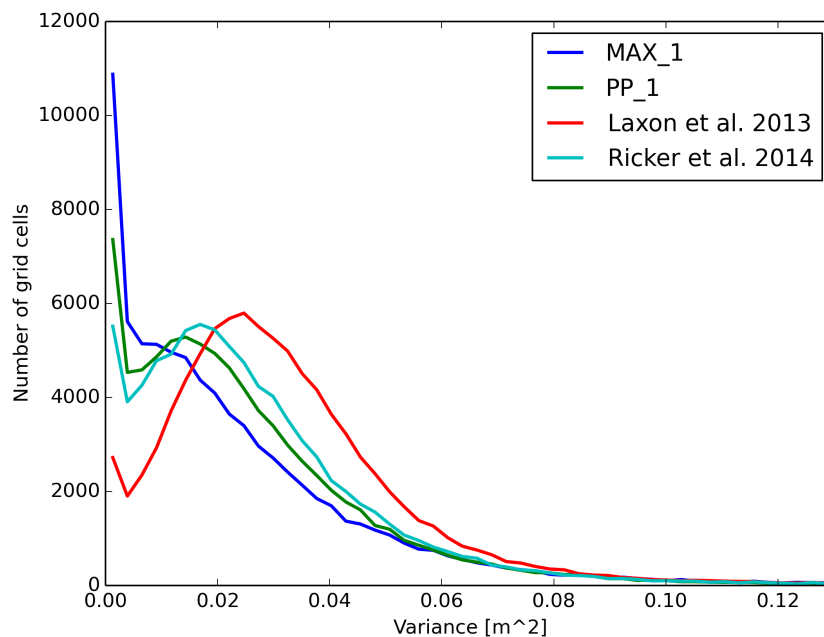
Fig. 1. Variance distribution
