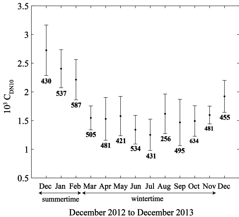
Fig. 1. Fig. 1 - Monthly median values of profile-derived from December 12, 2012 to December 30, 2013. The error bars are the one-fold interquartile range of the monthly data. The number under each dot corres
