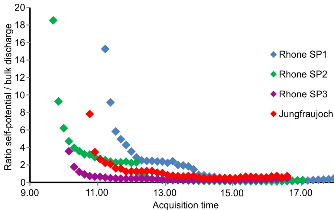
Fig. 4. Figure 3: Ratio between self-potential (V) and bulk discharge ( \text{m}^3 \text{s}^{-1} ) for each of the four surveys through time, illustrating the ratio changes consistently over time.
