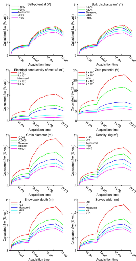
Fig. 3. Figure 6: Sw calculations for a range of values for each input parameter, using Rhone SP2 as an example.
