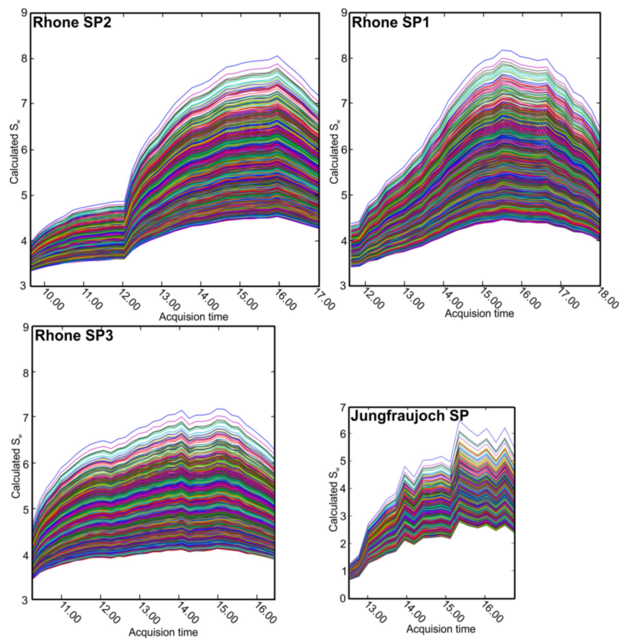
Fig. 1. Figure 7: Full sensitivity analysis for all 4 data sets.
