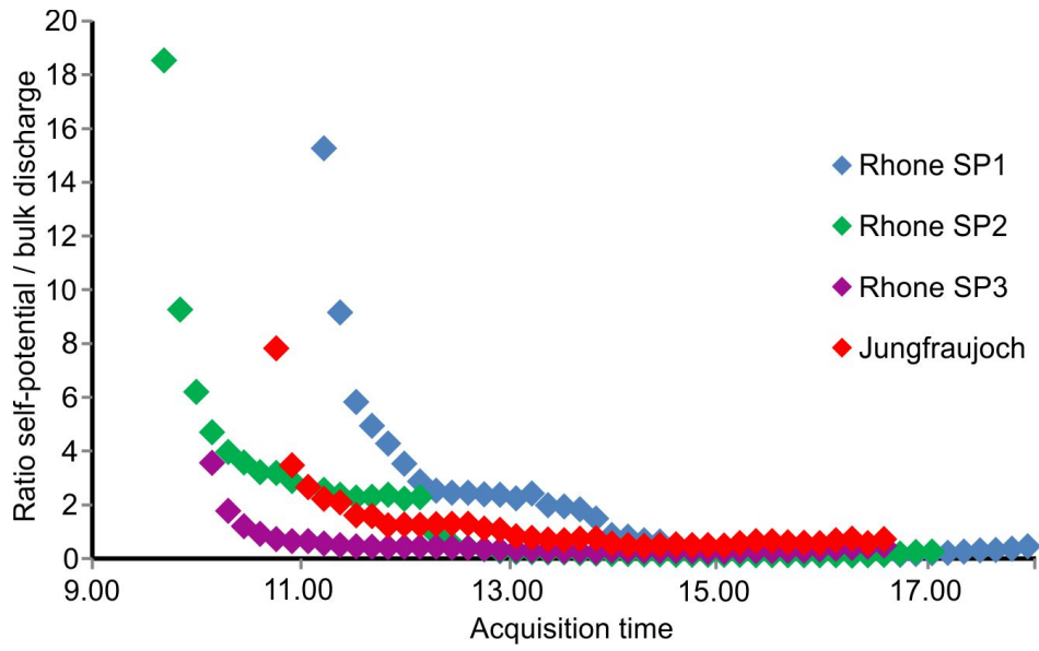
Fig. 4. Figure 3: Ratio between self-potential (V) and bulk discharge (m 3 s -1 ) for each of the four surveys through time, illustrating the ratio changes consistently over time.
