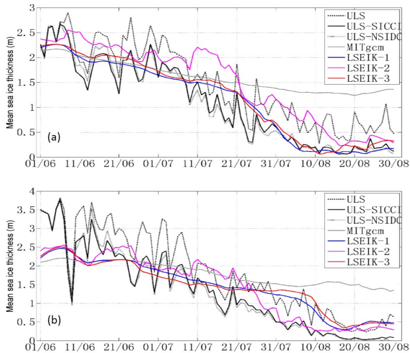
Fig. 2. Evolution of mean sea ice thickness (m) at (a) BGEF_2009A and (b) BGEF_2009D Beaufort Sea from 1 June to 30 August 2010. The black dotted lines show the original ULS thickness.
