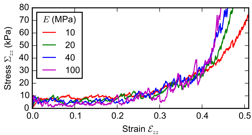
Fig. 2. Computed stress-strain curves for different Young's moduli.
