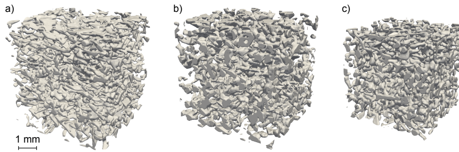
Fig. 1. Example of different snow microstructural patterns used in this study: (a) sample s-DF, (b) sample s-FCDH and (c) sample s-RG0. The size scale is the same for the three images.
