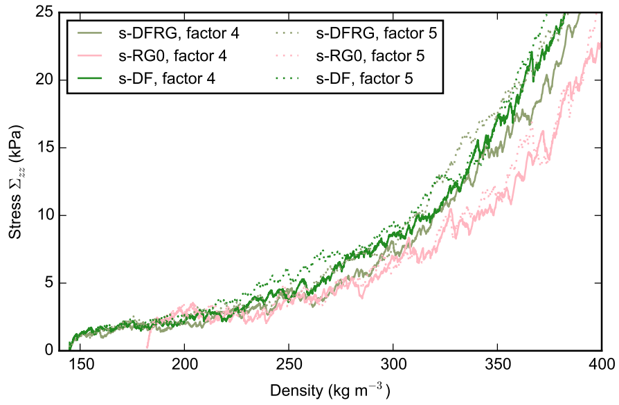
Fig. 3. Simulated stress-density relation for the samples s-DF, s-DFRG and s-RG and two different factors (4 and 5) of resolution reduction.
