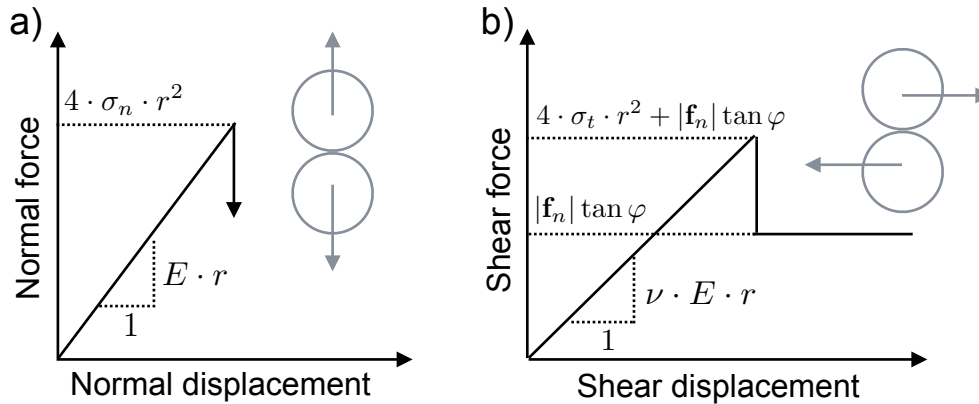
Fig. 1. Behavior of a sphere-sphere contact in two simple cases: normal loading (a) and simple shearing under constant normal force \mathbf{f}_n (b).
