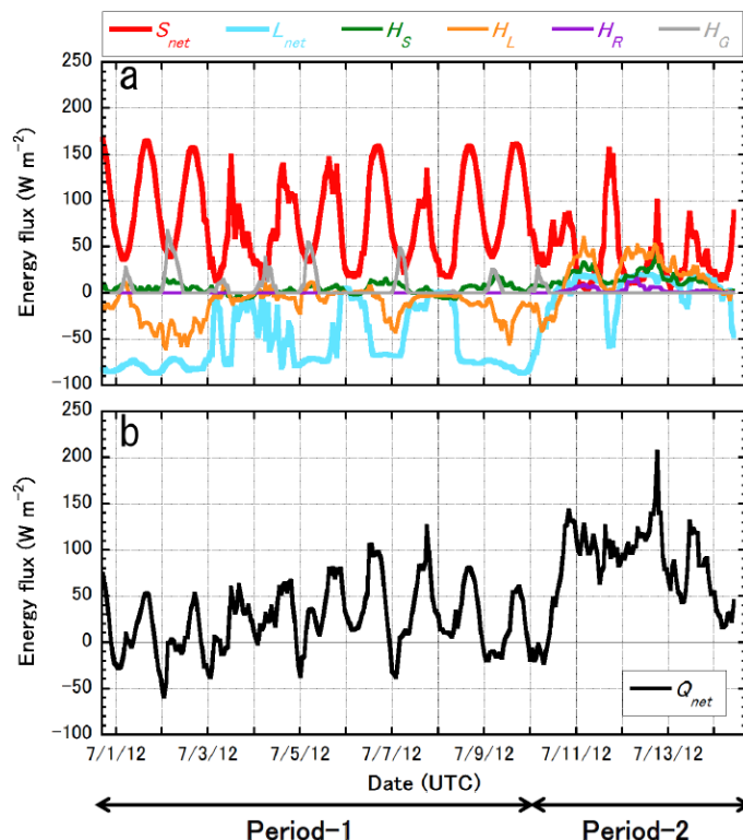
Figure 11. One-hour averaged surface energy balance at the SIGMA-A site during the IOP. The upper panel (a) shows net shortwave radiant flux ( S_{\text{net}} ), net longwave radiant flux ( L_{\text{net}} ), sensible heat flux ( H_S ), latent heat flux ( H_L ), heat supply by rainfall ( H_R ), and subsurface conductive heat flux ( H_G ). These fluxes are defined to be positive when they are directed into the snow surface. The lower panel (b) denotes net energy flux ( Q_{\text{net}} ). The snow surface is heated when Q_{\text{net}} is positive, whereas it is cooled if Q_{\text{net}} is negative.
