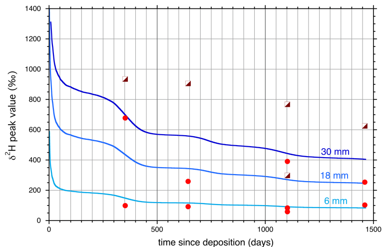
Figure 8. The actual peak height fits of the profiles (red circles). They are compared to the numerical simulations with initial layer thicknesses of 6, 18 and 30 mm, for which the diffusion length is fitted to the experimental points in Fig. 7. All experimental points are in the range spanned by the numerical calculations. The values for the ice layers that we removed from our profiles are also indicated (half-filled squares): all but one lie outside the possible range for diffused firn profiles, identifying them once more as ice layers.
