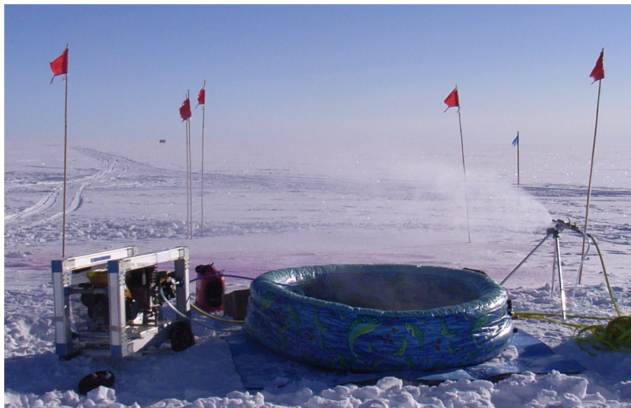
Figure 1. The production of the ^2\text{H} -labeled layer of snow at Summit, 8 August 2007. From left to right the air compressor/water pump rack, the inflatable water container and the snow gun.
