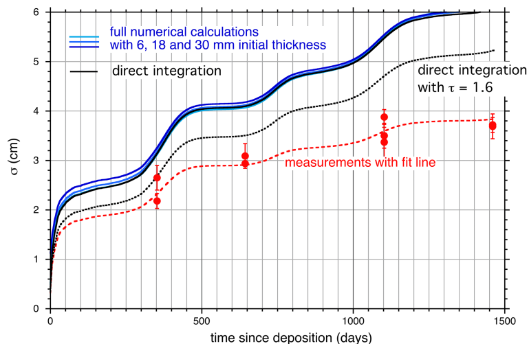
Figure 7. The results for the diffusion length \sigma . The points are the experimental results. The set of four higher-lying curves (one black, three in shades of blue) are the results of the numerical simulation using the Johnsen et al. (2000) model. The black one is the direct calculation of \sigma , the three blue ones result from the full numerical procedure starting with an enriched layer with 6, 18 and 30 mm initial thickness, respectively. Clearly, there is a systematic mismatch between the experimental results and the numerical simulations, increasing with time. The fit curve through the measurements is constructed by lowering the diffusivity by 25% in the first year, up to 40% in the last. Finally, the black dotted line shows the numerical result using a fixed, higher value for \tau (1.6).
