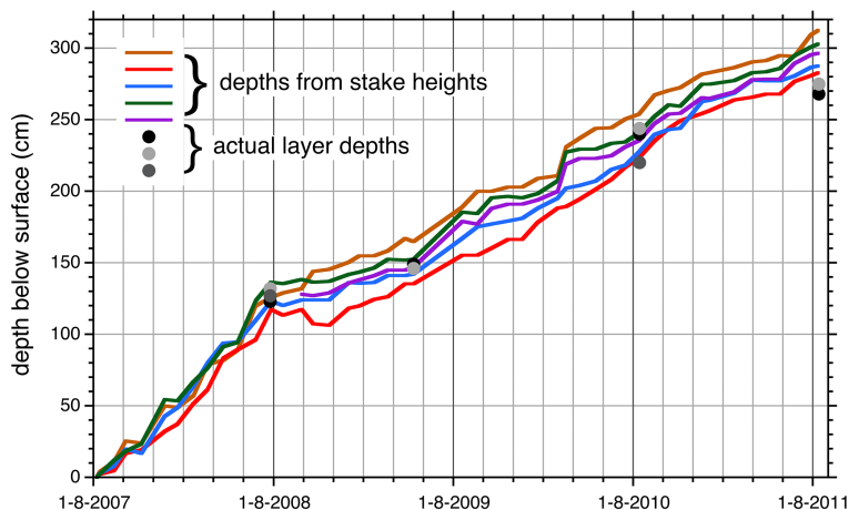
Figure 2. The depth of the enriched snow layer as a function of time, based on measuring the height of each of the 5 poles that mark the field (lines), together with the points indicating the actual depth of the enriched layer as revealed by the isotope measurements later in the lab (two to three points per year).
