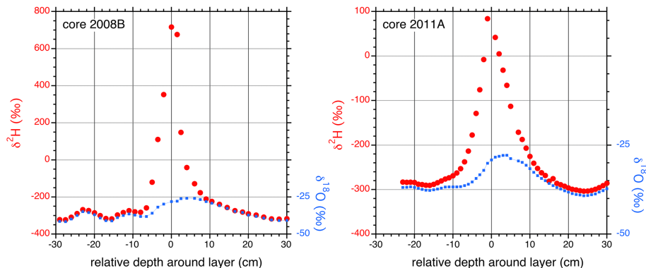
Figure 5. Two examples of \delta^2\text{H} profiles obtained in this work, from 2008 (core B), and from 2011 (core A), respectively. The effect of diffusion is directly visible, both in the width of the peak, and in its height. The \delta^{18}\text{O} signal is shown in blue, with scale ratio 1 : 8 with respect to the \delta^2\text{H} scale.
