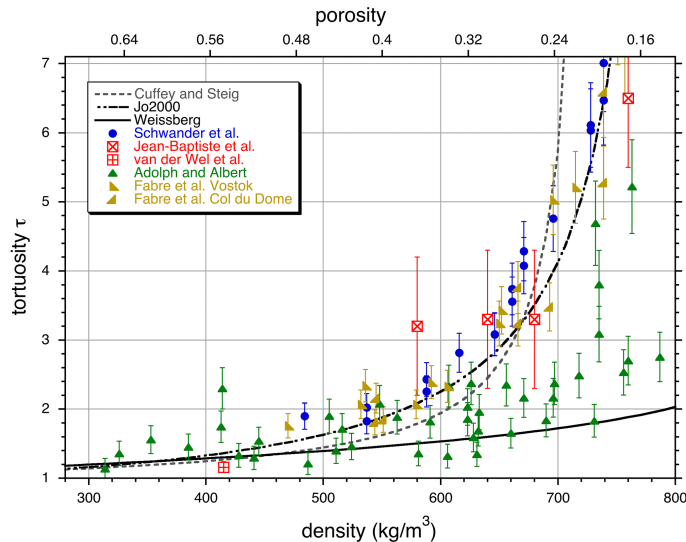
Figure 9. Results of various tortuosity measurements from literature, with \tau defined according to our Eq. (1). The symbols are the results of the various measurements: the red squares are laboratory firn diffusion measurements (by Jean-Baptiste et al., 1998 and van der Wel et al., 2011), the blue circles \text{CO}_2 and \text{O}_2 gas diffusion measurements through firn from Siple dome, Antarctica (Schwander et al., 1988), the green triangles \text{SF}_6 gas diffusion measurements through firn from Summit (Adolph and Albert, 2013, 2014). Finally pale brown triangles are the results by Fabre et al. (2000) for \text{SF}_6 gas diffusion in Vostok and Col du Dome. The black dash-dotted line is the parameterization for the Schwander et al. (1988) data in the Johnsen et al. (2000) model. The grey dashed curve is the tortuosity that is equivalent to the fit that Cuffey and Steig (1998) made to isotope seasonal cycles in the Summit firn layer. Furthermore, as a lower limit, we have included the theoretical result, interpreted as \tau , by Weissberg (1963), which he derived for spheres that can partly overlap or even fuse. For discussion of the results, see text.
