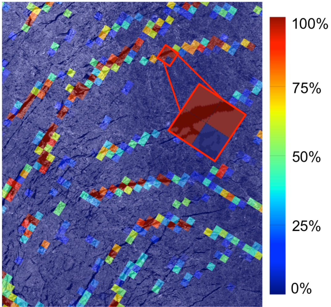
2 Figure 5. Subset of a SAR image taken on the 8 March 2009 overlaid by collocated AMSR-E 3 lead fraction (LF) product, where red grid cells correspond to LF 100% (for the other values 4 see the colour scale on the right). The zoom-in inset shows four grid cells where three of 5 them have AMSR-E LF 100% and one has LF 0%.
