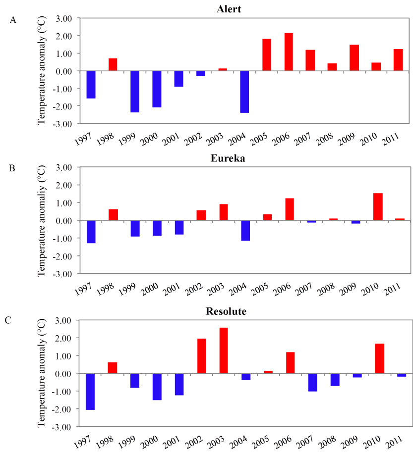
Figure 3. Air temperature anomalies for (a) Alert, (b) Eureka and (c) Resolute relative to the 1997–2011 mean annual temperature.
