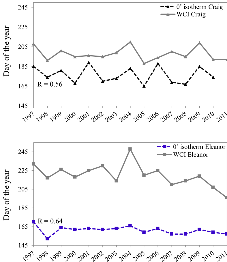
Figure 8. Water-clear-of-ice dates relative to the 0°C spring isotherm date between 1997 and 2011 for (a) Craig Lake (polar oasis) and (b) Eleanor Lake (polar desert). Spearman's rank correlation coefficient ( R ) is also shown.
