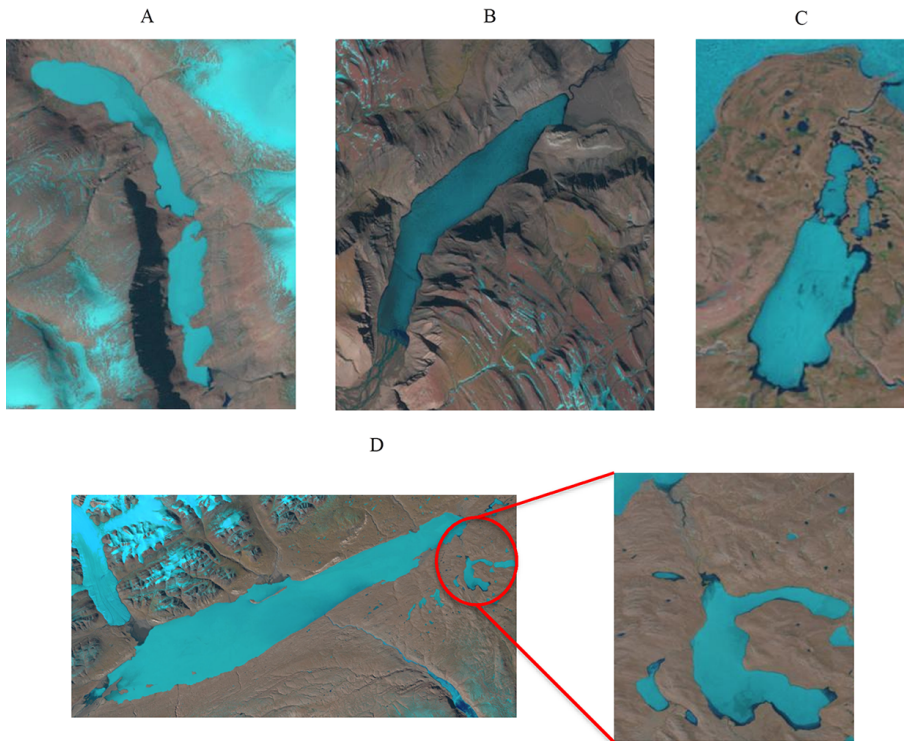
Figure 7. Landsat images acquired at the start of ice break-up showing melt and/or open water adjacent to water inflows: (a) Upper and Lower Murray Lakes (17 June 2007); (b) Buchanan Lake (8 July 1999); (c) Lake L6, (10 July 2003); (d) Lake Hazen and Craig Lake (16 June 2001).
