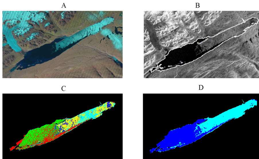
Figure 2. SAR-image segmentation processing steps: (a) landsat image of Lake Hazen, 19 July 2010; (b) original ASAR image of Lake Hazen acquired on 19 July 2010; (c) K means classified image (five clusters); (d) two-class map of ice (light blue) and open water (dark blue). The white line in the original SAR image represents the lake polygon that was used for defining the ROIs covering the lake.
