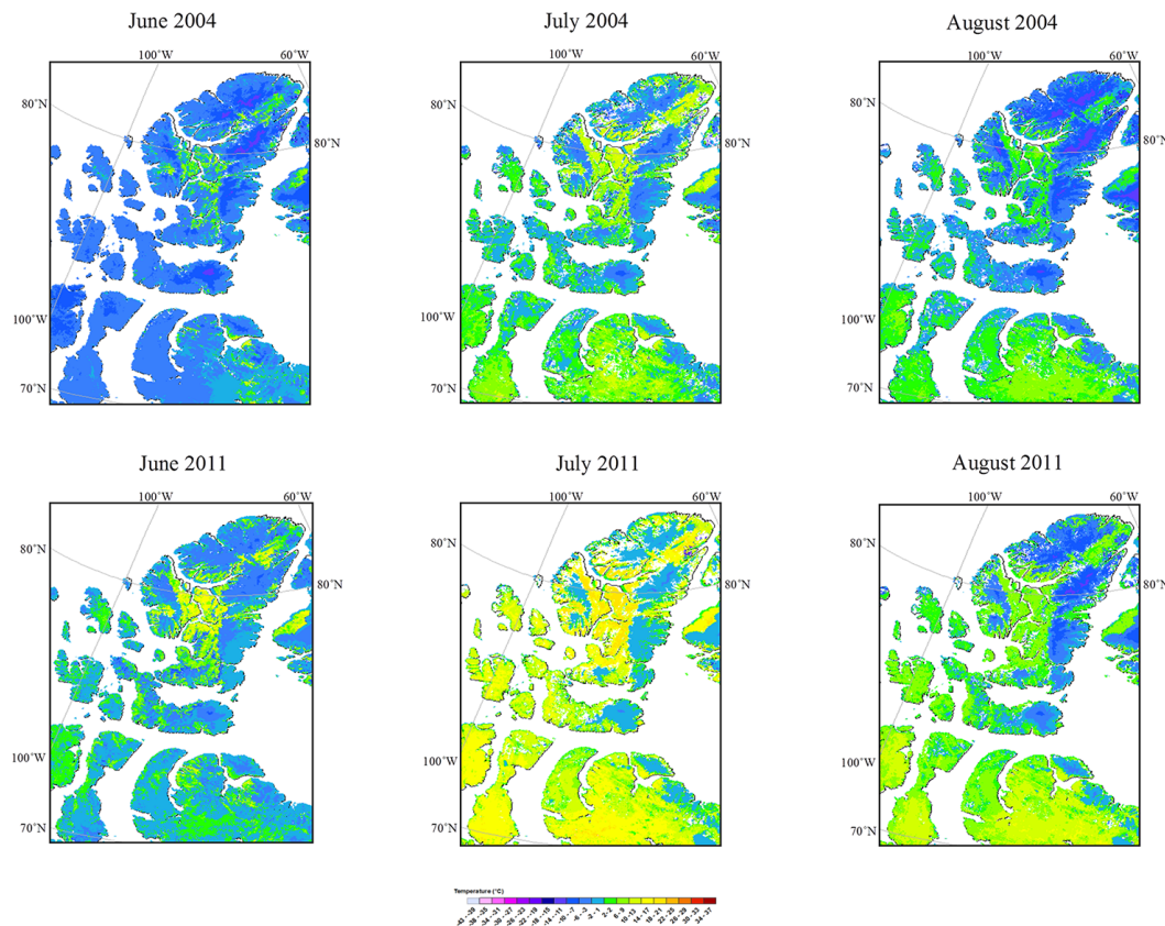
Figure 11. Mean land surface temperature derived from MODIS-Aqua/Terra over the Central/Eastern CAA during the months of June, July and August of 2004 (colder year) and 2011 (warmer year).
