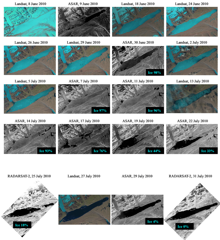
Figure 9. Time series of combined satellite observations (Landsat, ASAR and RADARSAT-2) for Lake Hazen during the break-up period of 2010. RADARSAT-2 Data and Products ©MacDonald, Dettwiler and Associates Ltd., 2010 – All Rights Reserved. RADARSAT is an official trademark of the Canadian Space Agency. Ice fractions for available SAR images are also shown. No ice fractions are shown for Landsat observations as image segmentation was only performed on SAR imagery.
