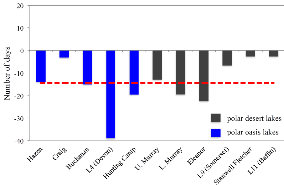
Figure 4. Changes – shown as number of days – in the melt onset date of investigated lakes in the Central and Eastern Canadian High Arctic (1997–2011). Number of days change is reported relative to the 1997–2011 mean melt onset day derived from spaceborne observations during this period. Lakes in polar oasis environments are shown as blue bars and lakes in polar desert environments are shown as grey bars. The red line indicates the 1997–2011 mean number of days change for melt onset.
