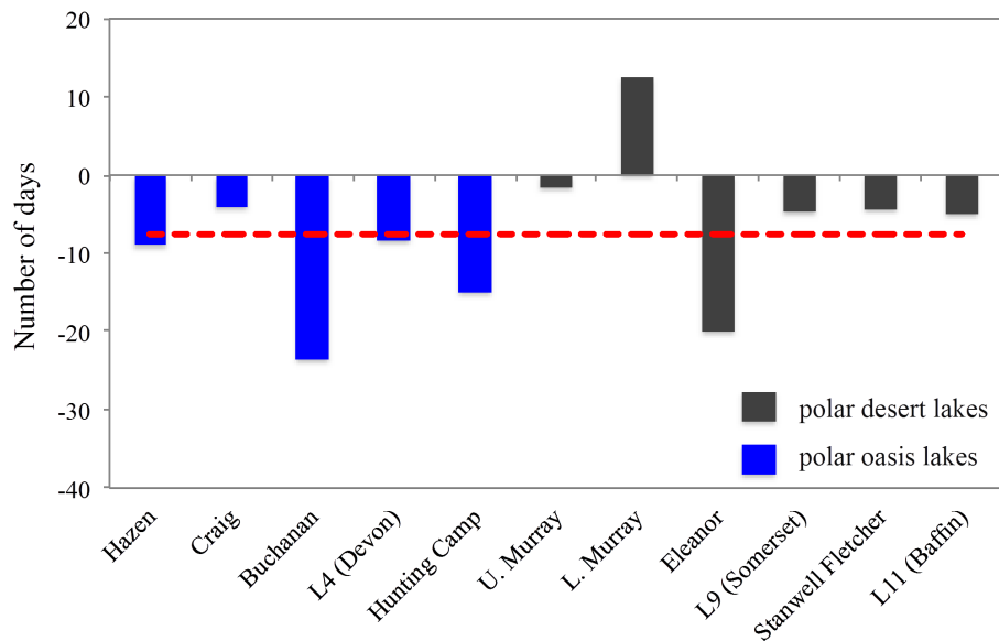
Figure 6. Changes – shown as number of days – in the water-clear-of-ice date of investigated lakes in the Central and Eastern Canadian High Arctic (1997–2011). Number of days change is reported relative to the 1997–2011 mean water-clear-of-ice day derived from spaceborne observations during this period. Lakes in polar oasis environments are shown as blue bars and lakes in polar desert environments are shown as grey bars. The red line indicates the 1997–2011 mean number of days change for water-clear-of-ice.
