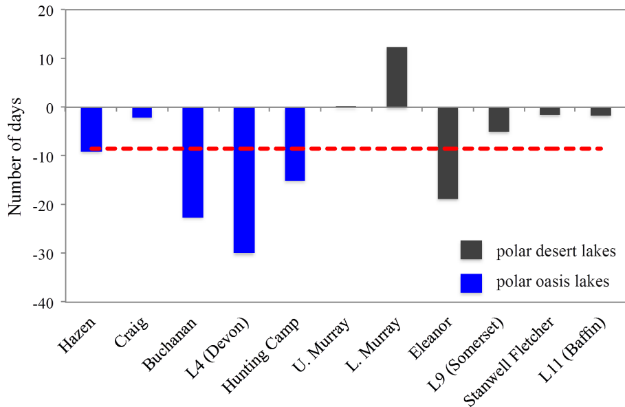
Figure 5. Changes – shown as number of days – in the summer ice minimum date of investigated lakes in the Central and Eastern Canadian High Arctic (1997–2011). Number of days change is reported relative to the 1997–2011 mean summer ice minimum day derived from spaceborne observations during this period. Lakes in polar oasis environments are shown as blue bars and lakes in polar desert environments are shown as grey bars. The red line indicates the 1997–2011 mean number of days change for summer ice minimum.
