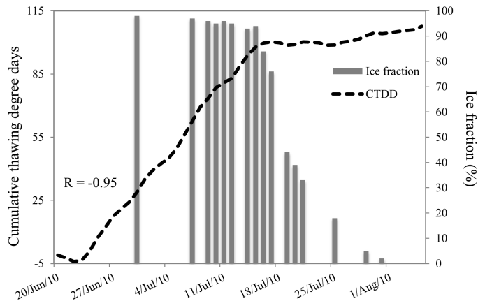
Figure 10. The cumulative thawing degree days and ice fraction for Lake Hazen during the 2010 break-up season.
