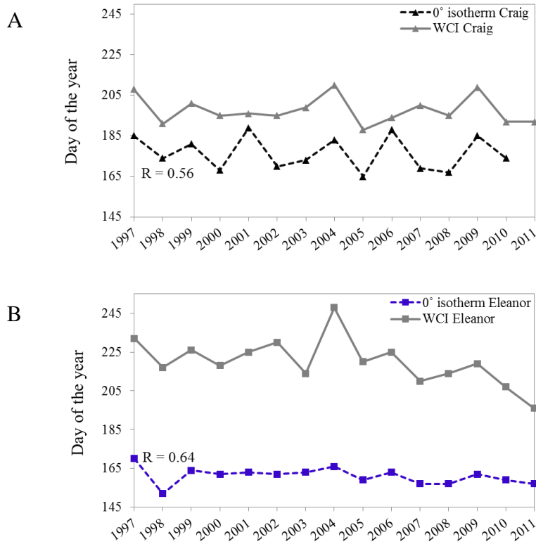
Fig. 8. Water-clear-of-ice dates relative to the 0°C spring isotherm date between 1997-2011 for (A) Craig Lake (polar oasis) and (B) Eleanor Lake (polar desert). Spearman’s rank correlation
