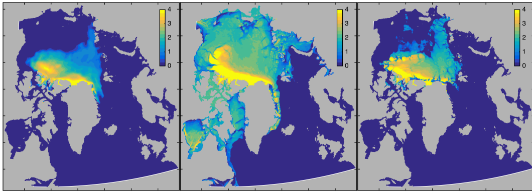
Figure 16. Ice thickness for the initial conditions (left panel), the model state at mid-winter (centre panel), and the model state at observed extent minimum (right panel). Note the increasing heterogeneity in the sea ice thickness field emerging from the new physics included in the model.
