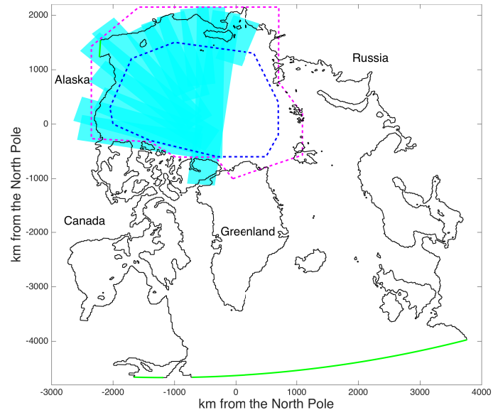
Figure 1. Model domain projected on a polar stereographic plane with open boundaries in green. The region delimited by the dashed blue line and the cyan area are used to compute the drift and deformation statistics. The dashed line in magenta shows the area for which the mean ice thickness and ice volume time series are calculated.
