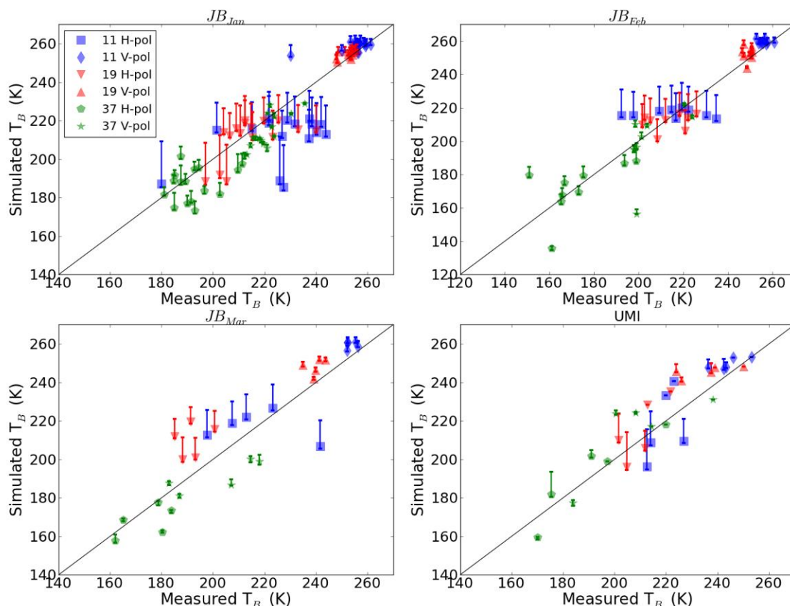
652 653 Fig. 11. T_B sensitivity associated with the \rho_{IL} variation ( 700 to 917 kg\ m^{-3} ). 654
