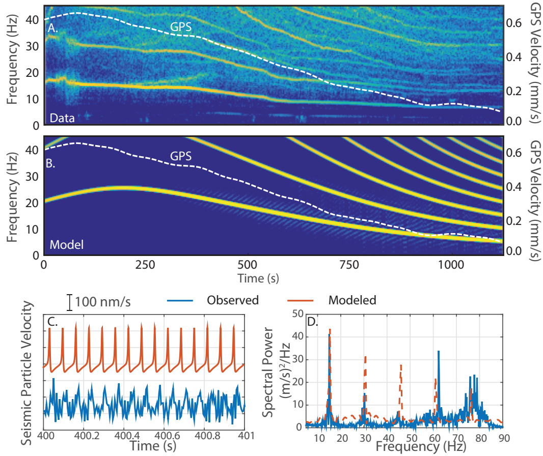
Figure 3. Comparison between observed (A.) and modeled (B.) tremor episode spectrograms for the episode that occurred on 2011-01-14 at 11:31. The white dashed line is the observed GPS velocity. The logarithmic color scales in both spectrograms are the same and have units of power spectral amplitude (\text{m/s})^2/\text{Hz} . The data were high pass filtered above 1 Hz before creating the spectrograms. The spectrograms use an 800 sample window with 50% overlap. We compare the modeled (red) and observed (blue) seismic velocity trace in (C.) and frequency spectrum in (D.). The frequency spectrum in (D.) is calculated over four second time windows for both the data and the model. Spectral bands from other, lower amplitude tremor sources are also present in the data shown in (A.).
