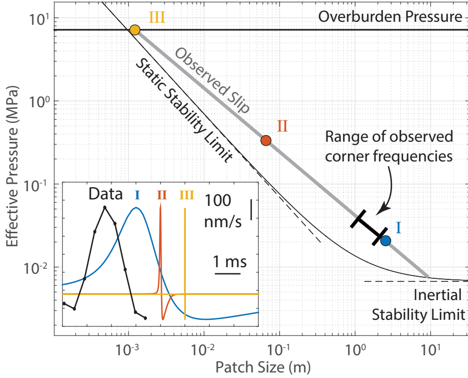
Figure 6. A diagram showing the range of patch size-effective pressure R - \bar{\sigma} conditions that give rise to fault slip D_{obs} = 40 \mu\text{m/s} (thick grey line). This figure shows a snapshot of parameter space at one instance during a tremor episode; the full evolution of parameters is shown in Figure 5. The heavy grey line shows the subset of parameter space that is also consistent with observed corner frequencies. The fault is loaded with velocity V_s = 0.4 \text{ mm/s} . The lower thin curve shows the boundary of the stability region Eq. (17). The horizontal line shows the overburden stress \rho_i g H . The inset shows a representative wave pulse recorded at high rate at station GS07 on 2010-12-14 as compared to three simulated wave forms. The bed shear modulus G_b for the simulations is chosen from Fig. 5 to be 15 MPa. Each simulation has the same seismic amplitude and slip; they differ only corner frequency ( f_c \approx 30, 750, \text{ and } 4000 \text{ Hz} ).
