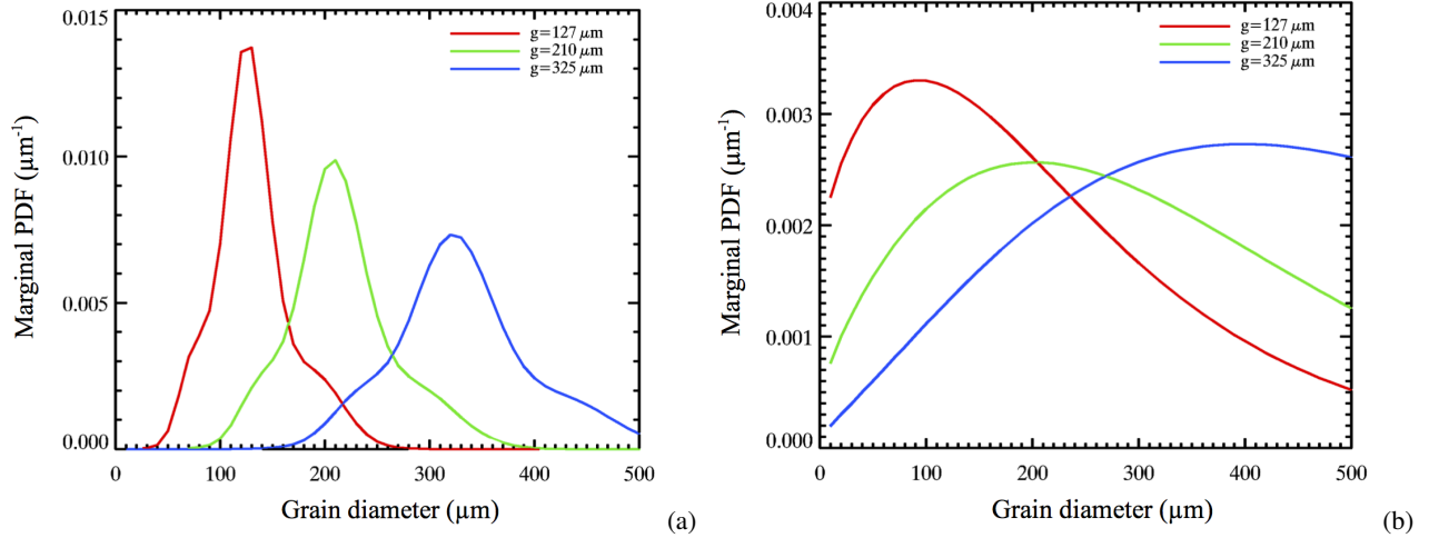
Figure 4. Normalized stacks of 1000 a posteriori PDF for the grain diameter of the snow, when conducting the inversion on synthetic data, with added random noise. The legends indicate the values for the grain diameter used to create the synthetic data. (a) The ice layer is 1 mm thick. (b) The ice layer is 5 mm thick.
