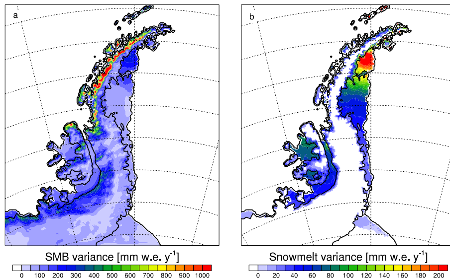
Figure 8. Interannual variability (one standard deviation, detrended) of SMB components for 1979–2014: SMB (a), and snowmelt (b), in mm weyr -1 .
