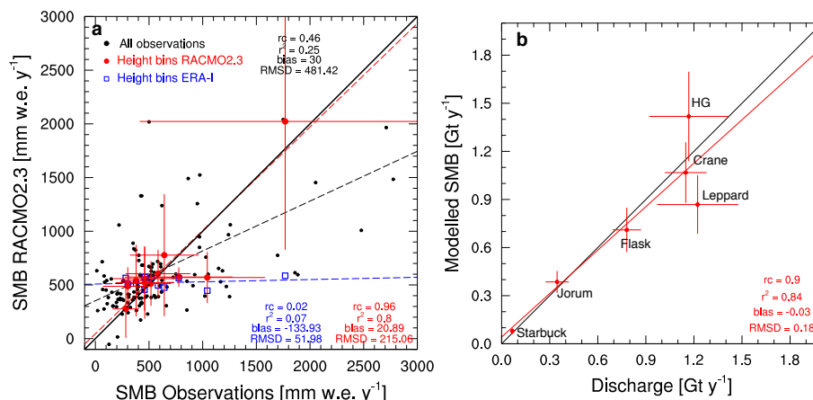
Figure 3. (a) Modelled SMB as a function of in-situ SMB observations (black dots), and the height bins as defined in Fig. 2 for RAMCO2.3 (red dots) and ERA-Interim (blue squares) in \text{mm weyr}^{-1} . Error bars represent one standard deviation within the height bins. Dashed lines represent the linear regressions lines. Two locations with either observed or modelled SMB values > 3000 \text{ mm weyr}^{-1} are off the chart and are not shown. Their respective (observed, modelled) SMB are (4200, 2658) and (660, 4908) \text{mm weyr}^{-1} . (b) Modelled SMB (with one standard deviation) as a function of drainage basins discharge estimates (with uncertainty) (Wuite et al., 2015) in \text{Gt yr}^{-1} . The red line represents the regression line of modelled SMB with discharge estimates.
