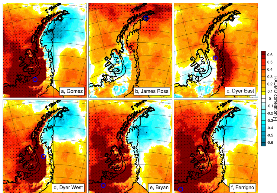
Figure 11. Correlation of modelled yearly (1979–2014) SMB at locations of Gomez (a, 73^{\circ} S, 70^{\circ} W), James Ross Island (b, 64.12^{\circ} S, 57.54^{\circ} W), Dyer Plateau East (c, 70.4^{\circ} S, 64.5^{\circ} W), Dyer Plateau West (d, 70.7^{\circ} S, 64.9^{\circ} W), Bryan Coast (e, 74.3^{\circ} S, 81.4^{\circ} W) and Ferrigno (f, 74.3^{\circ} S, 86.5^{\circ} W) ice cores, with all other points in the model domain. Stippled pattern represents significant correlations > 99\% . Locations of ice cores are denoted by blue circles. Note that over the sea-ice/ocean \text{SMB} = \text{PR} - \text{SU} .
