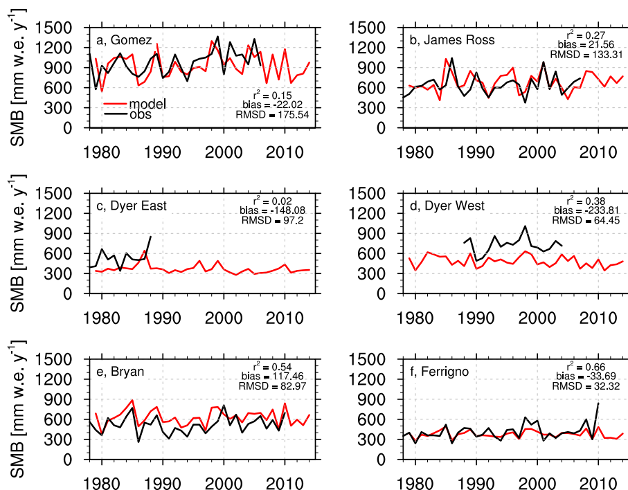
Figure 4. Modelled and observed yearly (1979–2014) SMB (mm we yr -1 ) at locations of Gomez (a, 73° S, 70° W), James Ross Island (b, 64.12° S, 57.54° W), Dyer Plateau East (c, 70.4° S, 64.5° W), Dyer Plateau West (d, 70.7° S, 64.9° W), Bryan Coast (e, 74.3° S, 81.4° W) and Ferrigno (f, 74.3° S, 86.5° W) ice cores. Statistics ( r^2 , bias and RMSD) are also given.
