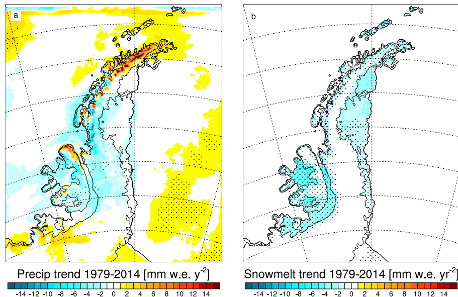
Figure 9. 1979–2014 trends of precipitation (a) and snowmelt (b) in mm we yr -2 . Stippled pattern represents trends that are significant > 95 %.
