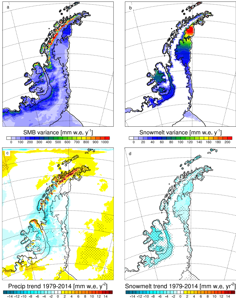
Fig. 8. Interannual variability (one standard deviation, detrended) of SMB components for 1979–2014: SMB (a), and snowmelt (b), in \text{mm w.e. yr}^{-1} . 1979–2014 trends of precipitation (c) and snowmelt (d) in \text{mm w.e. yr}^{-2} . Stippled pattern represents trends that are significant > 95%.
