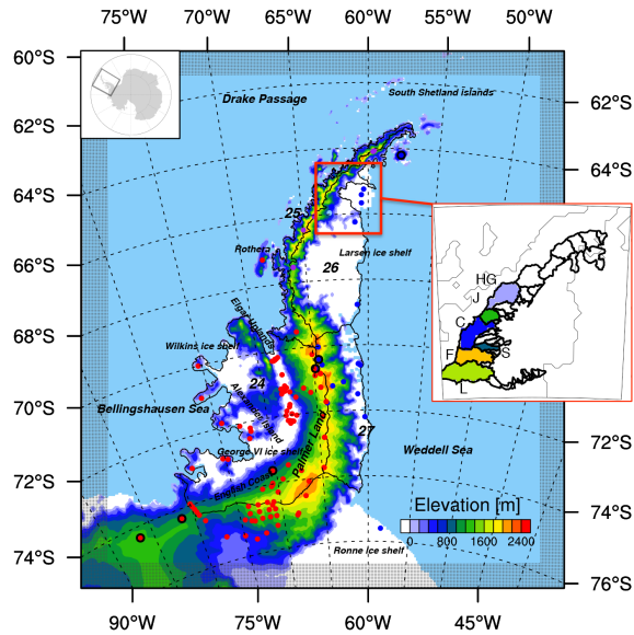
Fig. 1. RACMO2.3 Antarctic Peninsula model domain (black box in inset map of Antarctica), boundary relaxation zone (dotted area, 16 grid points) and model surface topography (m). Locations of in-situ SMB observations are marked (dots); ice cores, as used in Sect. 3.2, are highlighted (black circles). Colors of the dots indicate whether the observation lies in a WAP (red), EAP (blue) or spine (purple) height bin (see Sect. 3). Model topography is based on digital elevation models from Cook et al. (2012) for the region north of 70° S, and Bamber and Gomez-Dans (2009) south of 70° S. White areas represent floating ice shelves, colors represent the elevation of the grounded ice sheet. Zwally et al. (2012) drainage basins 24, 25, 26 and 27 are shown (black lines). One EAP in-situ observation is shown in light blue for visibility. Inset denotes the 6 drainage basins of pre-acceleration Larsen B outlet glaciers: Starbuck (S), Flask (F), Leppard (L), Crane (C), Jorum (J) and Hektoria-Green (HG) from Wuite et al. (2015).
