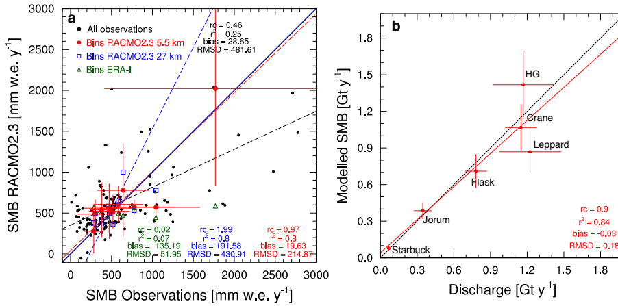
Fig. 3. (a) Modelled RACMO2.3 SMB at 5.5 km as a function of in-situ SMB observations (black dots), and the height bins as defined in Fig. 2 for RACMO2.3 5.5 km (red dots), RACMO2.3 27 km (blue squares) and ERA-Interim (green triangles) in \text{mm w.e. yr}^{-1} . Error bars represent one standard deviation within the height bins (for clarity error bars for RACMO2.3 27 km and ERA-Interim are not plotted). Dashed lines represent the linear regressions lines. Two locations with either observed or modelled SMB values > 3000 \text{ mm w.e. yr}^{-1} , as well as one binned 27 km location, are off the chart and are not shown for clarity. (b) Modelled RACMO2.3 SMB at 5.5 km (with one standard deviation) as a function of drainage basins discharge estimates (with uncertainty) (Wuite et al., 2015) in \text{Gt yr}^{-1} . The red line represents the regression line of modelled SMB with discharge estimates. Basin locations are shown in Fig. 1.
