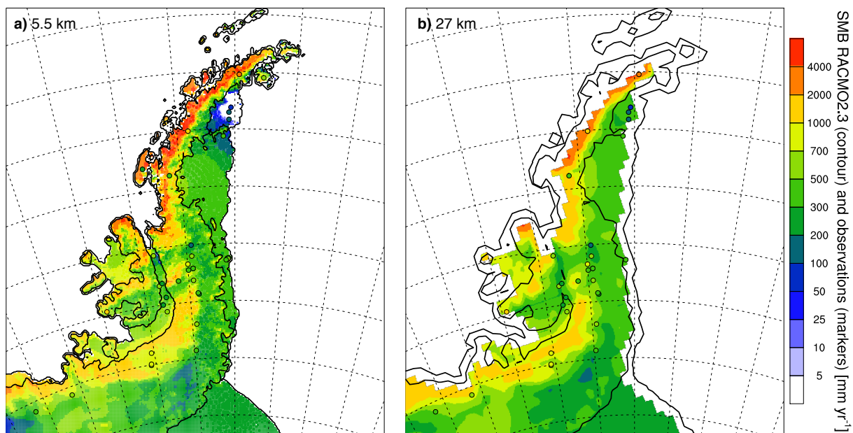
Fig. 6. Modelled SMB (colours) and observations (markers) in \text{mm weyr}^{-1} at 5.5 km (a) and 27 km (b) horizontal resolution (Van Wessem et al., 2014b). Observations are from Turner et al. (2002), Favier et al. (2013) and Scambos et al. (2014) and sources noted in Sect. 2.3, and only shown if they represent a period > 5 years. Modelled SMB is the 1979–2014 climatological average. At both resolutions only ice sheet grid points are shown.
