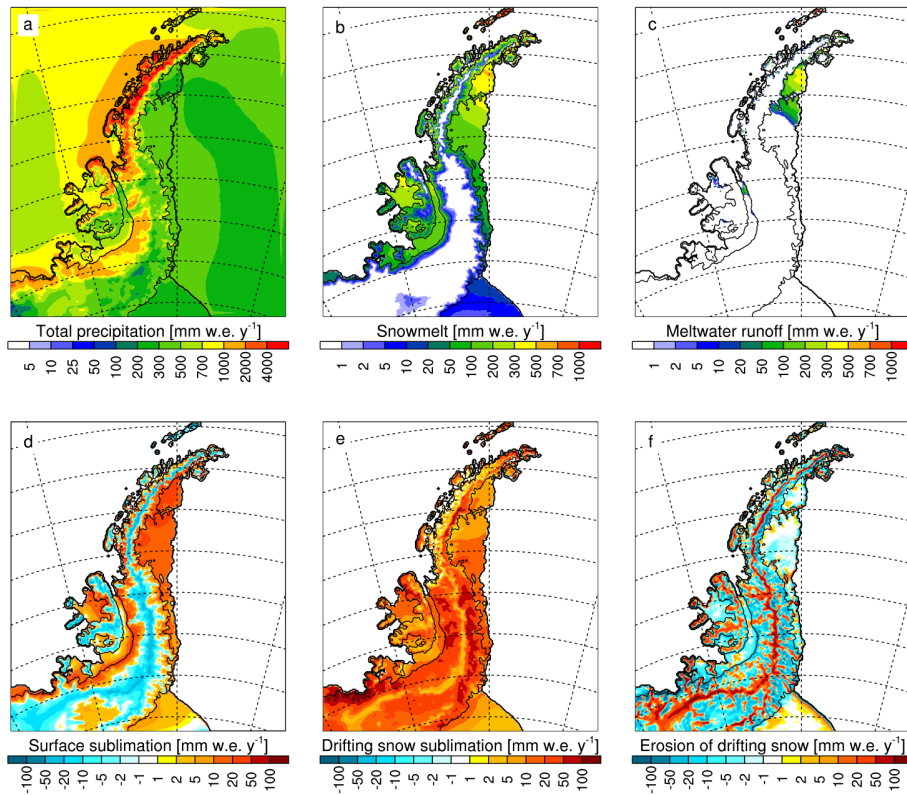
Fig. 5. 1979–2014 average SMB components: total precipitation (snowfall + rain) (a) , snowmelt (b) , meltwater runoff (c) , total sublimation (d) , sublimation of drifting snow (e) and erosion of drifting snow (f) in \text{mm w.e. yr}^{-1} . Note that ablation is defined positive in (d–f) . All fluxes are from RACMO2.3, except for runoff, which is calculated by the FDM that is forced by RACMO2.3 output.
