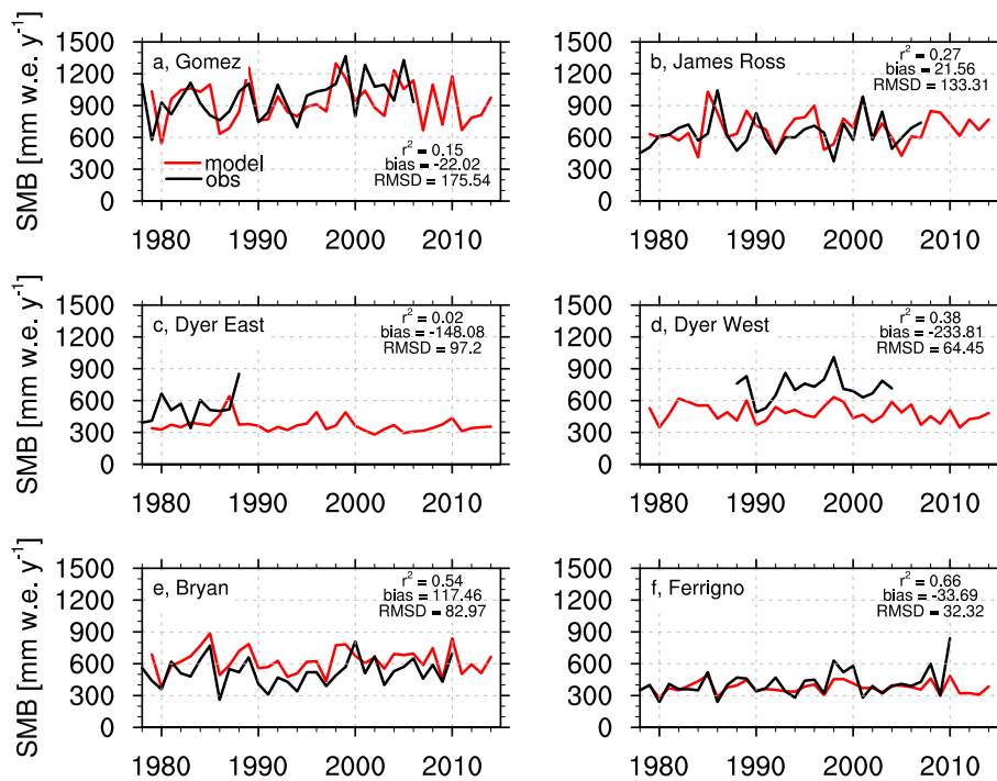
Fig. 4. Modelled and observed yearly (1979–2014) SMB ( \text{mm weyr}^{-1} ) at locations of Gomez ( a , 73^\circ \text{ S} , 70^\circ \text{ W} ), James Ross Island ( b , 64.12^\circ \text{ S} , 57.54^\circ \text{ W} ), Dyer Plateau East ( c , 70.4^\circ \text{ S} , 64.5^\circ \text{ W} ), Dyer Plateau West ( d , 70.7^\circ \text{ S} , 64.9^\circ \text{ W} ), Bryan Coast ( e , 74.3^\circ \text{ S} , 81.4^\circ \text{ W} ) and Ferrigno ( f , 74.3^\circ \text{ S} , 86.5^\circ \text{ W} ) ice core sites. Statistics ( r^2 , bias and RMSD) are also given. Ice core locations are shown in Figs. 1 and. 10
