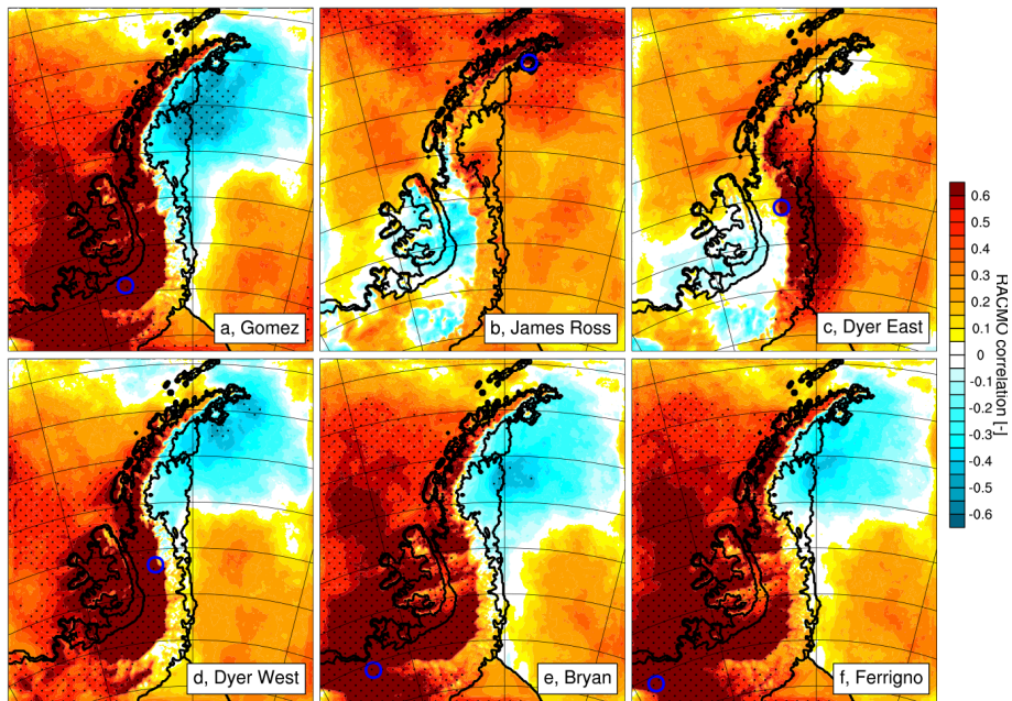
Fig. 10. Correlation of modelled yearly (1979–2014) SMB at locations of Gomez ( a , 73^{\circ} S, 70^{\circ} W), James Ross Island ( b , 64.12^{\circ} S, 57.54^{\circ} W), Dyer Plateau East ( c , 70.4^{\circ} S, 64.5^{\circ} W), Dyer Plateau West ( d , 70.7^{\circ} S, 64.9^{\circ} W), Bryan Coast ( e , 74.3^{\circ} S, 81.4^{\circ} W) and Ferrigno ( f , 74.3^{\circ} S, 86.5^{\circ} W) ice cores, with all other points in the model domain. Stippled pattern represents significant correlations > 99\% . Locations of ice cores are denoted by blue circles. Note that over the sea-ice/ocean \text{SMB} = \text{PR} - \text{SU} .
