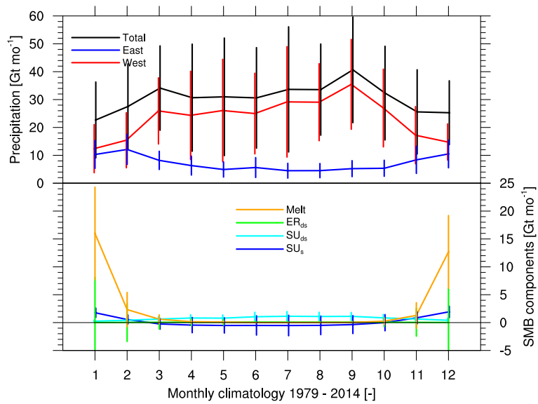
Fig. 9. 1979–2014 monthly climatology of SMB components: top panel shows total precipitation (snow-fall + rain) averaged for the WAP drainage basins (red line), the EAP (blue), and total (black). Bottom panel shows total (WAP + EAP) snowmelt (orange), erosion of drifting snow ER_{ds} (green), drifting snow sublimation SU_{ds} (cyan), and surface sublimation/deposition (blue). All variables in Gt\ mo^{-1} .
