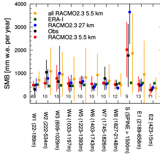
Fig. 2. Modelled RACMO2.3 5.5 km (red), RACMO2.3 27 km (blue), ERA-Interim (green) and observed (black) SMB as a function of eleven elevation bins for all in-situ SMB observations. The orange dots are the average SMB of all RACMO 5.5 km grid points in the elevation bins. The bins are arranged from west to east in three separate classes (WAP (W1–8), the spine (S) and the EAP (E1–2)), using the drainage basin definition from Zwally et al. (2012). Error bars represent one standard deviation within the bin and amount of observations in each bin is denoted within the plot. Further details are provided in the text (Sect. 2.3.1).
