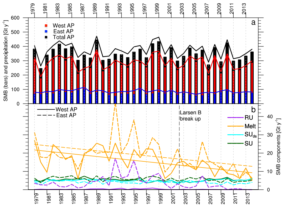
Fig. 7. Yearly average SMB (a) and SMB components (b) in \text{Gt yr}^{-1} . For SMB, values for the WAP (red) and the EAP (blue) are shown. SMB is integrated over basins 24, 25, 26 and 27 from Zwally et al. (2012). Trend lines are only shown if significant. From 2003 onwards integrated values represent the ice shelf excluding Larsen B ice shelf.
