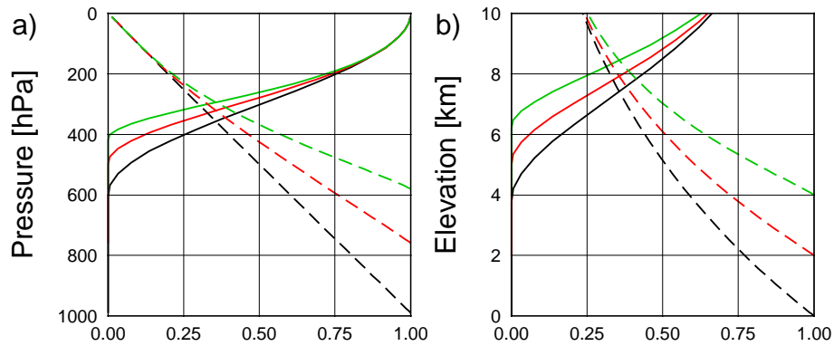
Fig. 1. \lambda_\sigma(\sigma) (solid lines) and \sigma (dashed lines) as function of (a) pressure and (b) elevation for a location at 0 (black lines), 2000 (red lines) and 4000 (green lines) m a.s.l., respectively.
