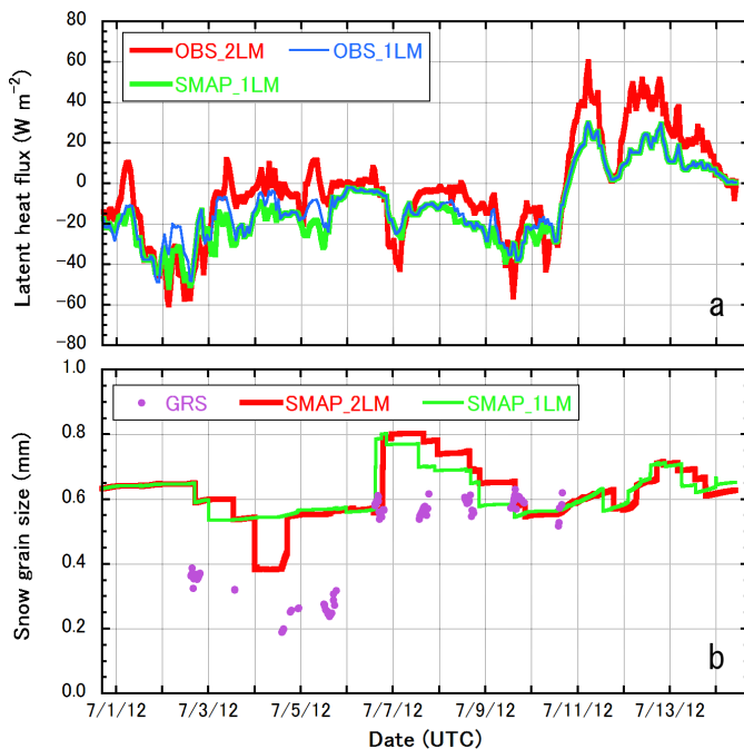
Figure 12. (a) Temporal evolution of 1 h averaged latent heat fluxes calculated from atmospheric measurements at 6 and 3 m above the surface (OBS_2LM) and measurements at 3 m above the surface (OBS_1LM), as well as the SMAP simulation forced by 1-level (3 m above the surface) atmospheric measurements (SMAP_1LM). (b) Comparison of surface snow grain size at the SIGMA-A site during the IOP with surface snow grain size from ground-based remote sensing (GRS) using spectral albedo data measured with a spectrometer and those from the SMAP simulations driven by 2-level (6 and 3 m above the surface) atmospheric measurements (SMAP_2LM) or 1-level (3 m above the surface) atmospheric measurements (SMAP_1LM).
