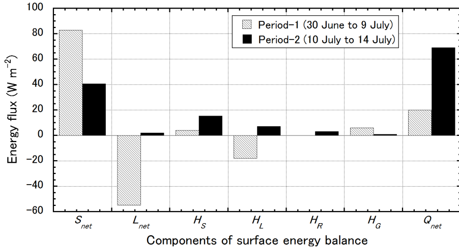
Figure 11. Comparison of average surface energy balance components ( S_{\text{net}} : net shortwave radiant flux, L_{\text{net}} : net longwave radiant flux, H_S : sensible heat flux, H_L : latent heat flux, H_R : heat supply by rainfall, H_G : subsurface conductive heat flux, and Q_{\text{net}} : net energy flux) between Period-1 and Period-2 at the SIGMA-A site.
