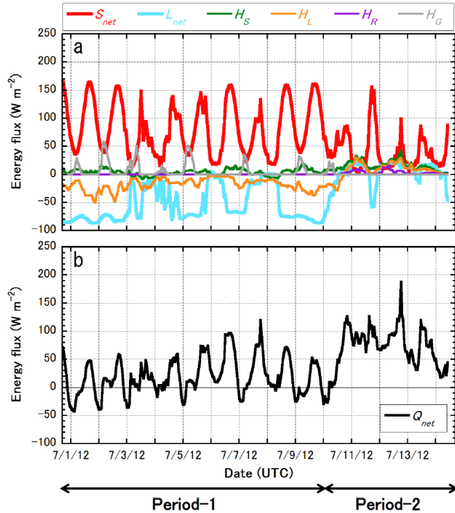
Figure 10. One-hour averaged surface energy balance at the SIGMA-A site during the IOP. The upper panel (a) shows net shortwave radiant flux ( S_{\text{net}} ), net longwave radiant flux ( L_{\text{net}} ), sensible heat flux ( H_S ), latent heat flux ( H_L ), heat supply by rainfall ( H_R ), and subsurface conductive heat flux ( H_G ). These fluxes are defined to be positive when they are directed into the snow surface. The lower panel (b) denotes net energy flux ( Q_{\text{net}} ). The snow surface is heated when Q_{\text{net}} is positive, whereas it is cooled if Q_{\text{net}} is negative.
