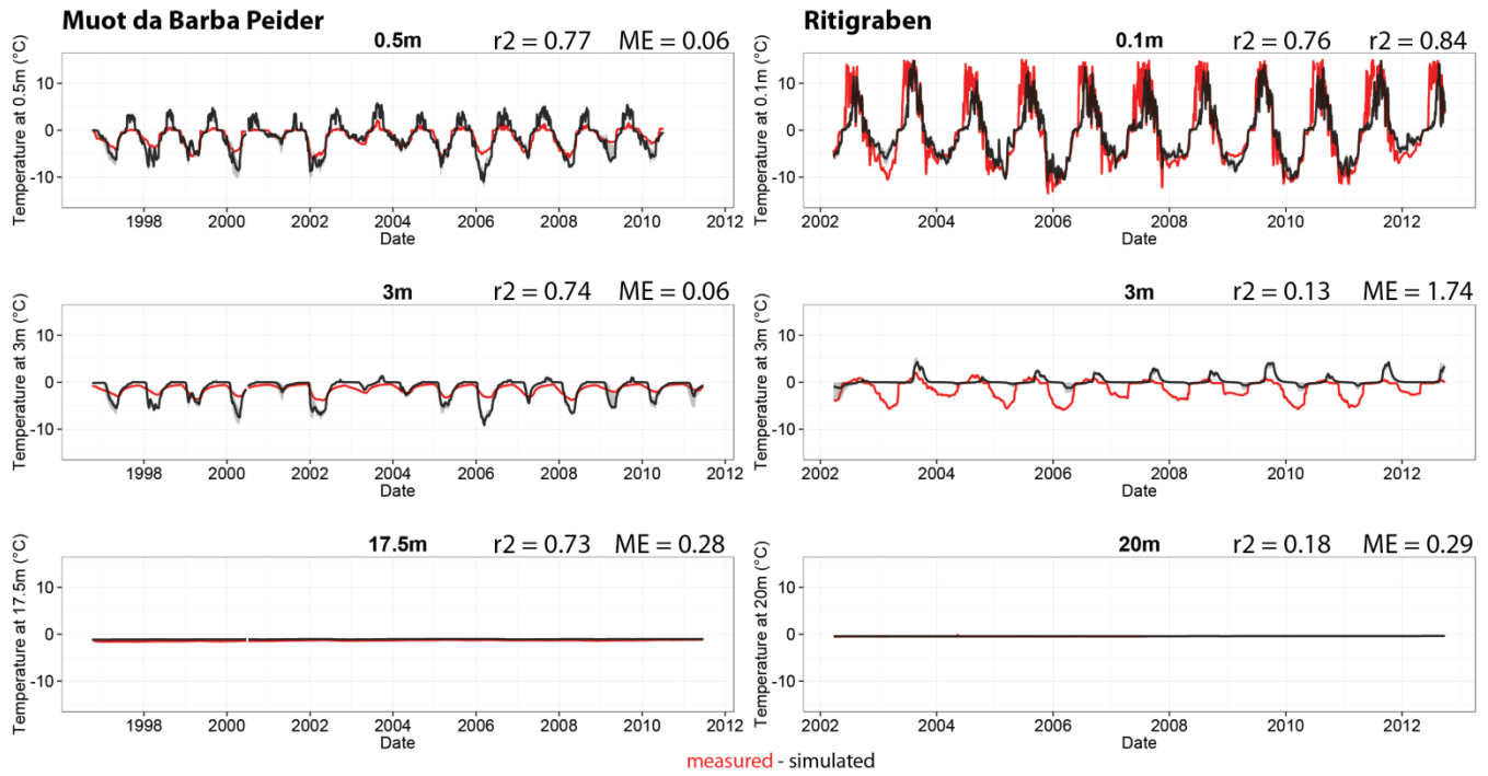
Figure 6b – Comparison of simulated (black) and measured (red) temperature during the calibration period at six sites at three different depths: one close to the surface, one around 3 m and one close to the lower boundary of the model for Muot da Barba Peider and Ritigraben.
