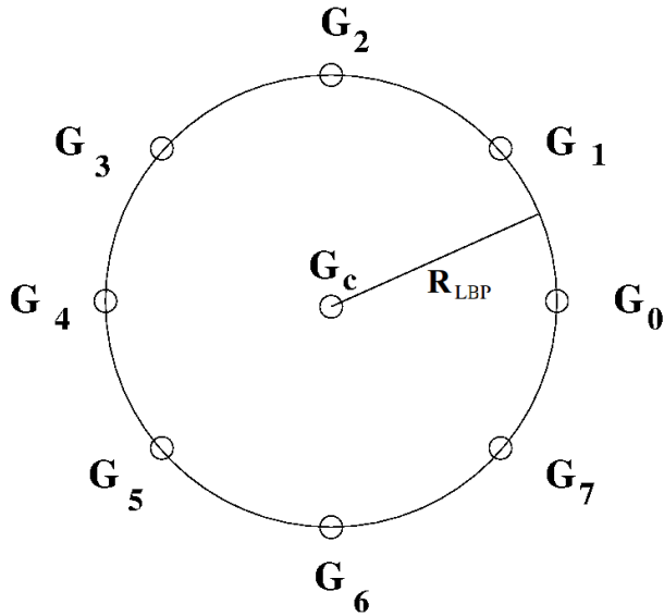
Figure 5. Geometry of an LBP with an angular step of \pi/4 . The circle has a radius of R , which is one LBP parameter.
