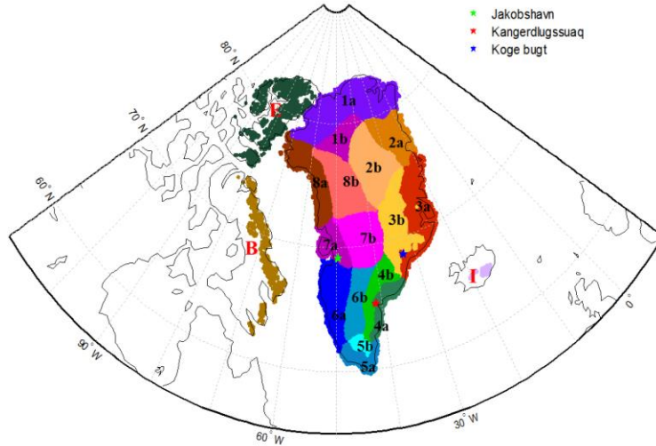
Figure 1. The GrIS mascon layout, based on the drainage system definition by Zwally (2012).
