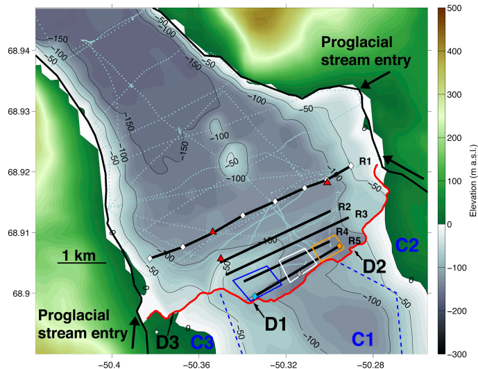
Figure 3. July 2012 Survey of Sarqardleq Fjord. Sarqardleq Fjord bathymetry (10 m colored contours below sea level within fjord) and Morlighem et al. (2014) bedmap (10 m colored contours above and below sea level outside of fjord) are shown. The Sarqardliup sermia front position and coastline from a 19 June 2012 Landsat image are mapped in red and black line, respectively. Depth measurements collected during July 2012 field operations used to create the Sarqardleq Fjord bathymetry are plotted as grey dots over the contoured bathymetry. RE-MUS transects R1–R5 are shown in black, with LBL transponders mapped with red triangles. Subglacial subcatchments C1, C2, and C3 dividing lines from MBM2014 analysis are mapped in dashed blue line, with the location of D1, D2, and D3 subglacial discharge channels along the submerged terminus shown with thin black arrows. CTD casts are shown with diamonds: white diamonds are CTD casts along R1 used in REMUS cross-calibration, and the blue, gold, and grey diamonds are CTD casts 1, 2, and 3 that were taken along R5 within GMW1, GMW2, and the region between GMW1 and GMW2 (outlined in blue, gold, and white, respectively). Three proglacial stream entries to Sarqardleq Fjord are shown along the northeast and southwest fjord coastlines with thick black arrows.
