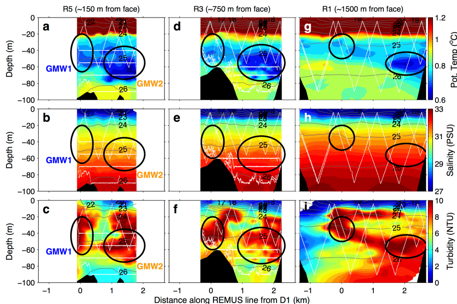
Figure 4. Select REMUS Across-Fjord Sections. \theta ( ^{\circ}\text{C} ), S (PSU), and turbidity (NTU) sections along REMUS lines R5 (a–c), R3 (d–f), and R1 (g–i) from 0 to 100 m depth. Sections are oriented looking away from the terminus, with the southwestern end of the section on the left. Across-fjord transect distance is plotted as horizontal distance along section, with 0 km located at the intersection of the REMUS section with an along-fjord line running from D1 to the southwestern LBL transponder along R1 (Fig. 3). GMW1 and GMW2 regions identified by black ellipses, and labeled in blue and gold, respectively in (a)–(c). Isopycnals plotted in grey, REMUS mission tracks shown in white (Table 1), and bathymetry shown in black (Fig. 3).
