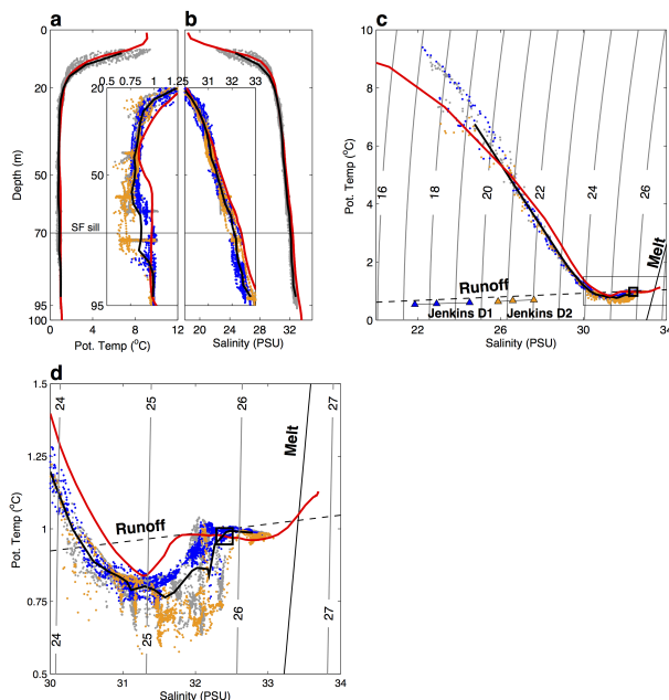
Figure 5. Glacially Modified Water in Sarqardleq Fjord. \theta ( ^{\circ}\text{C} ) ( a ) and S ( b ) profiles for R4 and R5 measurements over the full water-column depth (grey), with the average of R4 and R5 measurements and the ambient fjord waters in black and red, respectively. ( a ) and ( b ) insets show same data from 20–95 m depth over a finer \theta or S range, with measurements taken within the GMW1 and GMW2 regions along R4 and R5 (Fig. 3) shown in blue and gold, respectively. \theta/S plots of R4 and R5 measurements ( c ) (colors same as in a and b ), with melt and runoff mixing lines. Intersection for melt and runoff mixing lines set to CTD2 properties at grounding line depth (Fig. 6b). Black square along ambient fjord water profile shows \theta/S properties at sill depth (70 m). \theta/S results for the Jenkins (2011) plume modeling (Table 4) of D1 (blue triangles) and D2 (gold triangles) shown. ( d ) Same data as in ( c ) over finer \theta/S range indicated by thin black box in ( c ).
