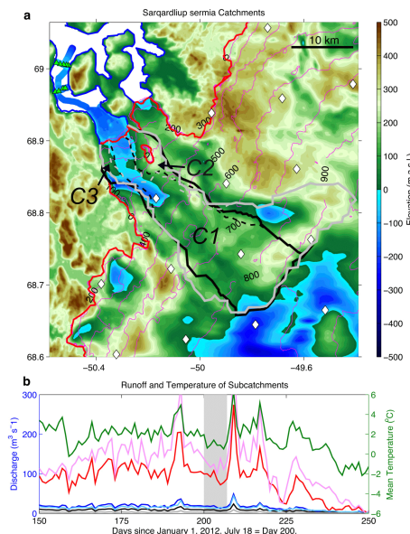
Figure 7. Sargardliup sermia catchments and discharge. (a) Estimated Sargardliup sermia catchment (thick black line) and sub-catchments C1, C2, and C3 (dashed black line) from the MBM2014 analysis over Morlighem et al. (2014) bedmap (filled contours) and ice sheet surface (magenta contours). BBM2013 catchment and subcatchments outlines in thick solid and dashed grey lines, respectively. Ice sheet margin and coastlines shown in red and blue, respectively. RACMO2.3 11 km resolution grid points shown with white diamonds. Sargardleq fjord bathymetry and outer Sargardleq fjord CTD positions (green triangles) and depth measurements also shown. (b) Daily C1, C2, and C3 subcatchment MBM2014 RACMO2.3 discharge estimates (red, blue, and black lines, respectively) and daily average RACMO2.3 temperature (green line) across the Sargardliup sermia subcatchment C1 for DOY 150–250, 2012. Daily C1, C2, and C3 subcatchment BBM2013 RACMO2.3 discharge estimates in pink, cyan, and grey lines, respectively. Dates of REMUS and CTD sampling from DOY 200–207 marked by grey bar.
