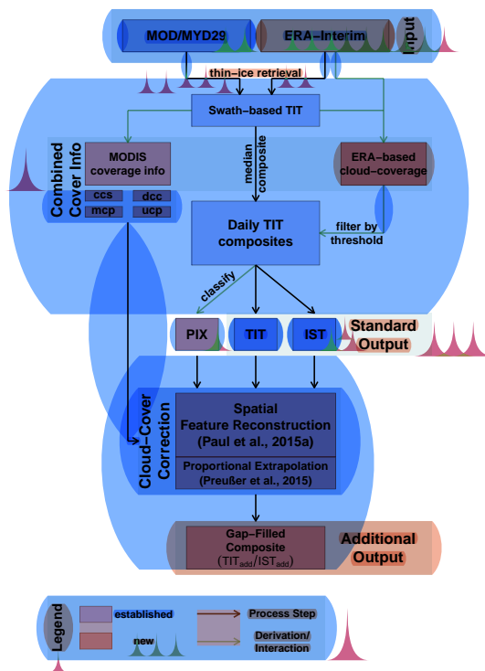
Figure 2. Work flow based on the described input data and thin-ice retrieval. Established processing steps, that were already used in other studies are marked in blue, while new additions are marked in red. These additions comprise a persistence index (PIX), the newly defined combined cloud-cover information of MODIS cloud mask and ERA-Interim medium-level cloud cover. Missing data due to cloud cover is accounted for by a two-step procedure that comprises spatial feature reconstruction (Paul et al., 2015a) and proportional extrapolation (Preußner et al., 2015). The combined cloud-cover information separates between confident clear-sky (ccs), definite cloud-cover (dcc), mixed-covered pixels (mcp) and uncovered pixels (ucp).
