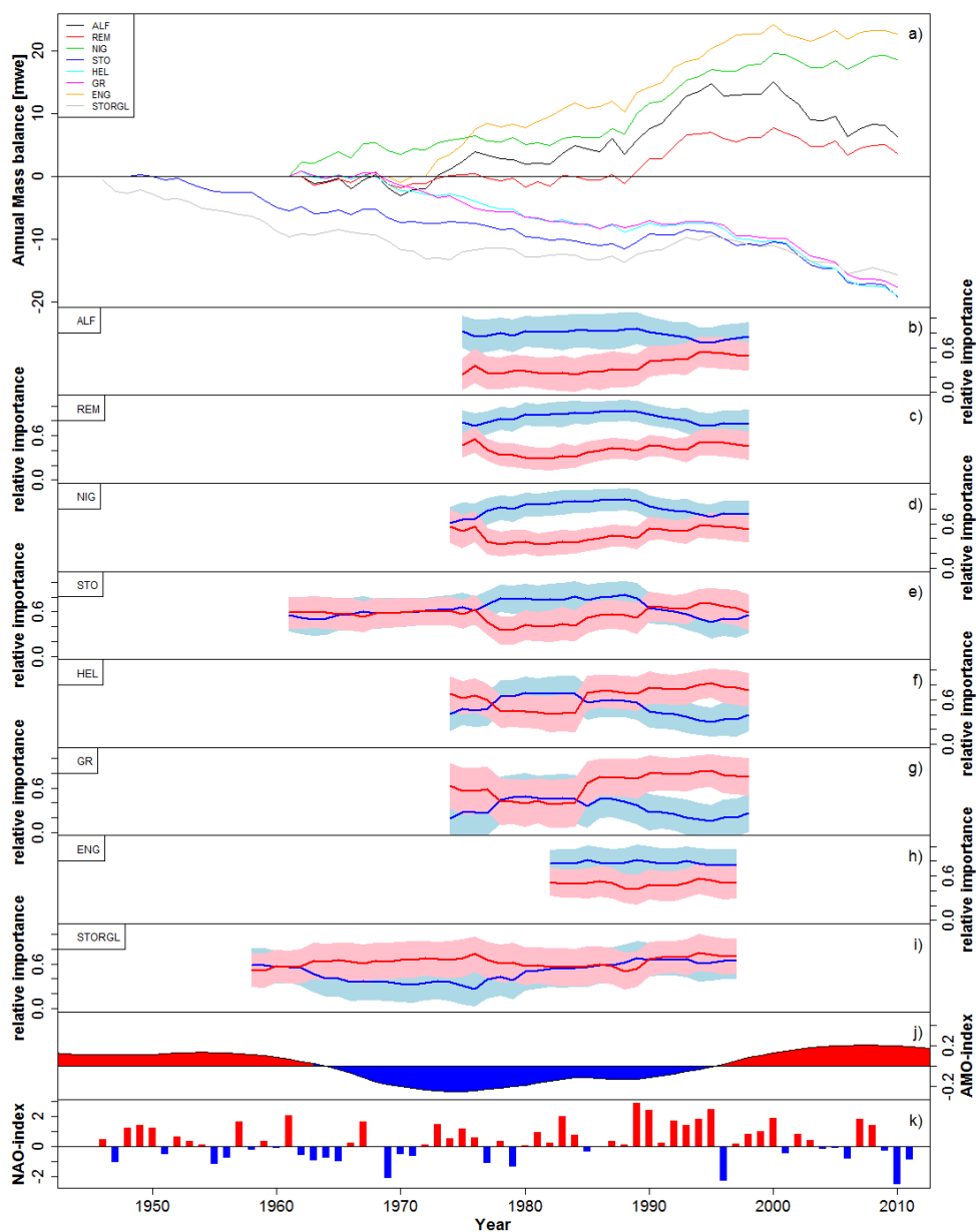
1 2 Figure 3. a) Cumulative mass balances of Ålfotbreen (ALF), Rembesdalsskåka (REM), 3 Nigardsbreen (NIG), Storbreen (STO), Hellstugubreen (HEL), Gråsubreen (GR), Engabreen 4 (ENG) and Storglaciären (STORGL). Data: nve.no/bre (Norwegian glaciers) and 5 bolin.su.se/data/tarfala (Storglaciären, northern Sweden).
