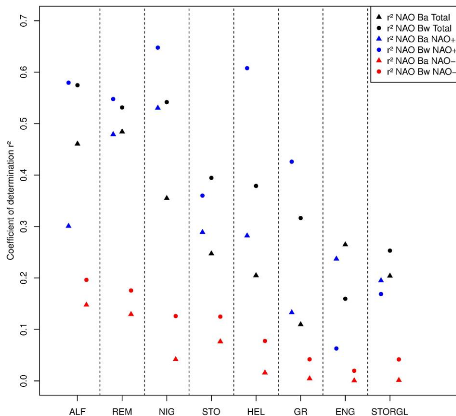
1 2 Figure 5. Coefficients of determination ( r^2 ) among mass balances and North Atlantic 3 Oscillation (NAO) Index (Jones et al., 1997, updated). Coefficients of determination between 4 winter mass balances and annual mass balances and winter NAO-index. Coefficients of 5 determinations are shown for the entire measurement period (central symbols) and for periods 6 of above (left symbols, blue ) and below (right symbols, red ) median NAO-index, 7 respectively. Bw: winter mass balance, Ba: annual mass balance; NAO: NAO-index.
