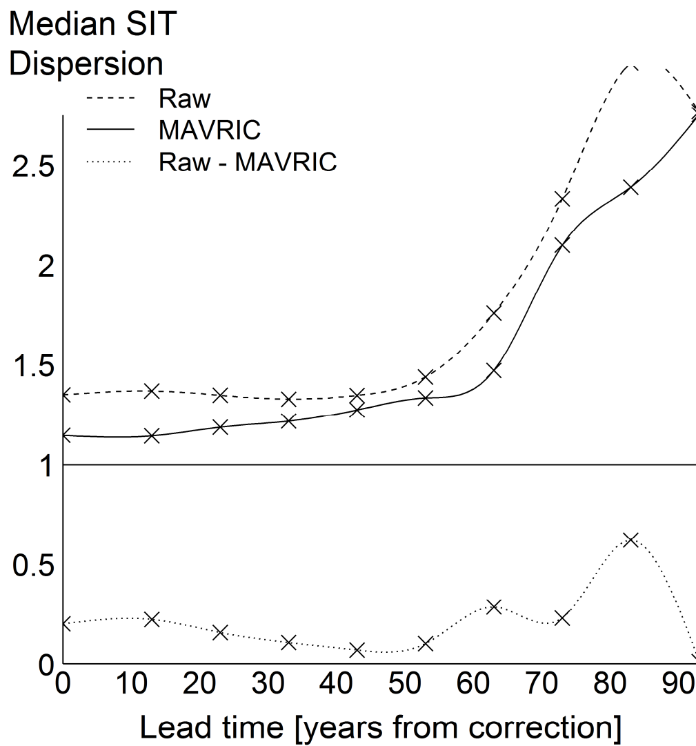
1 2 Figure C2. Multi-model ensemble out of sample September median SIT dispersion
