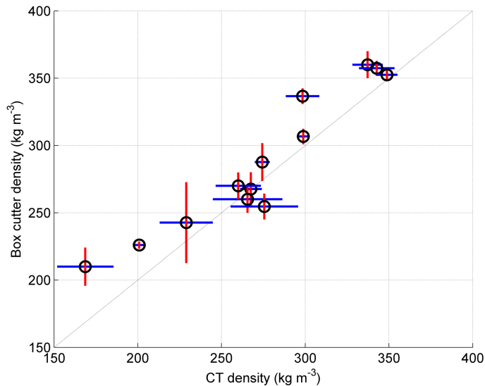
Figure 2 The three cutter measurements (0–9 cm) in each of 13 blocks were averaged to best match the location of the \mu CT samples. Error bars are \pm one standard deviation, resulting from these three cutter measurements (red) and the three \mu CT samples per block (blue).
