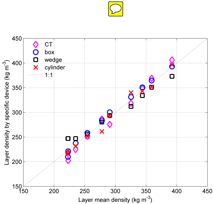
Figure 5. Different measurement methods averaged to match the traditional layers, vs. the mean layer density. Mean layer densities are the average of all layer densities of the different methods. Statistics are given in Table 6.
