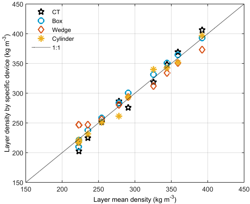
Figure 5. Different measurement methods averaged to match the traditional layers, vs. the mean layer density. Mean layer densities are the average of all layer densities of the different methods. Statistics are given in Table 6.
