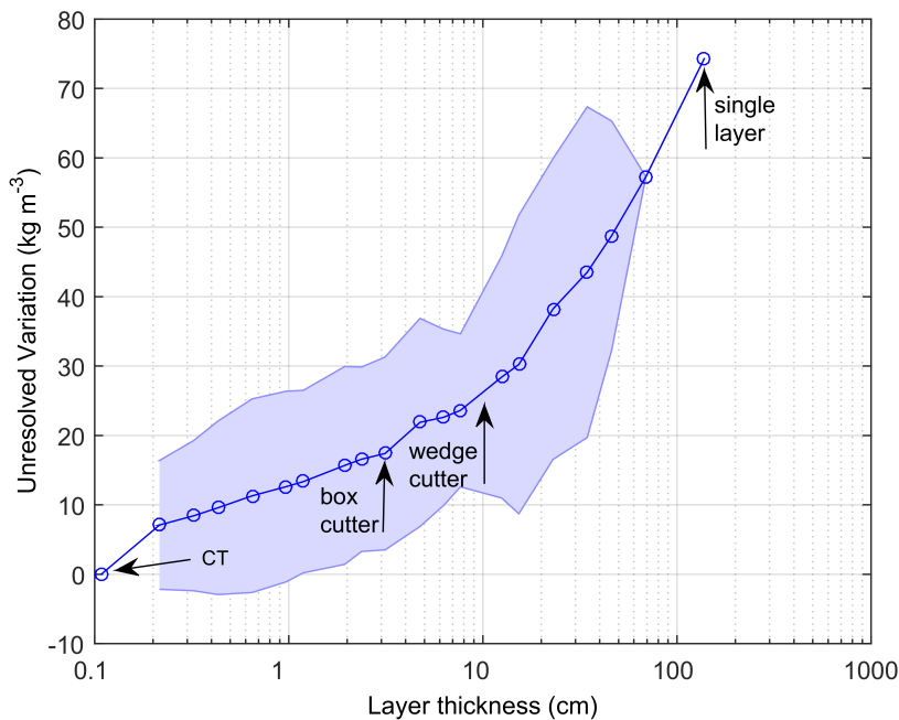
Figure 7. Unresolved variation of \mu\text{CT} profile vertically averaged to larger layer thickness, with the vertical resolution of box cutter (3 cm), wedge cutter (10 cm) and a single layer profile indicated. The shaded area indicates \pm one standard deviation.
