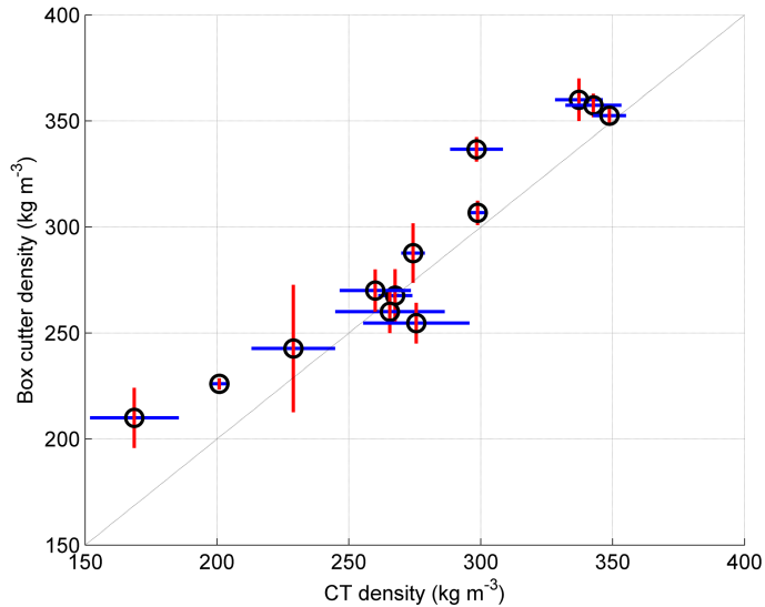
Figure 2. Comparison of density cutter and \mu CT measurements in the laboratory. The top three cutter measurements (0–9 cm) in each of the 13 blocks were averaged to best match the location of the \mu CT samples. Error bars are \pm one standard deviation, resulting from these three cutter measurements (red) and the three \mu CT samples per block (blue).
