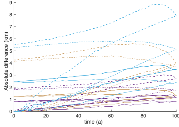
Figure 3. Experiment MISMIP3d P75S and P75R: evolution of the absolute differences in km between the highest resolution ( N_y = 80 ) and the two others ( N_y = 40 continuous line and N_y = 20 dashed line) for the three different methods: LG (brown), DI (purple) and FF (blue), on the symmetry axis ( y = 0 ; thick curves) and on the free-slip boundary ( y = 50 km; thin curves).
