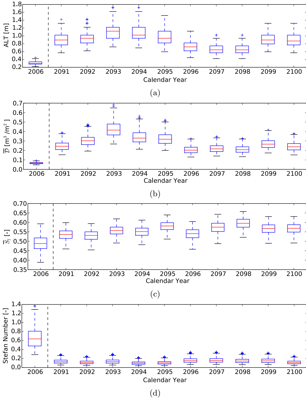
Figure 4. Boxplots of projected metrics including (a) ALT, (b) annual thaw depth-duration, (c) annual mean liquid saturation, and (d) Stefan number for year 2006 and from 2091 to 2100. The bottom and top of the boxes are the first and third quartiles, the red lines are medians, the whisker lengths are 1.5 times the interquartile range (50%), and the plus symbols are outliers.
