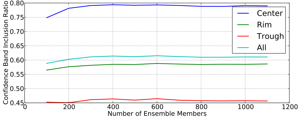
Figure 4. Calibration-constrained ensemble convergence analysis based on the ratio of measured temperatures from the BEO within the 95% confidence band for ensemble simulated temperatures.
