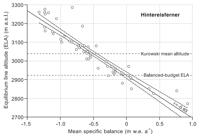
Figure 4. Equilibrium line altitude (ELA) plotted against mean specific mass balance of Hintereisferner, Austrian Alps. Dashed lines denote 95 % confidence interval around the regression line according to Student t statistic (Kreyszig, 1970, p. 302).
