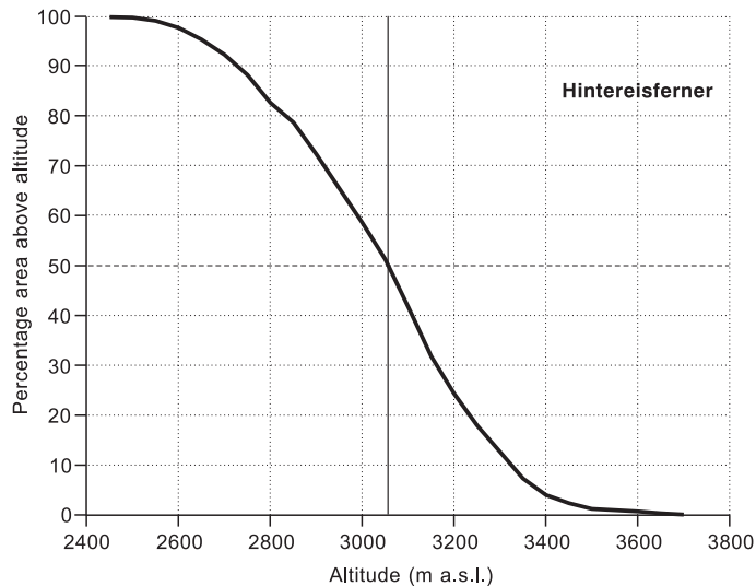
Figure 2. Hypsographic curve for Hintereisferner, Austrian Alps, showing the percentage of glacier area above any particular altitude. Area distribution is for year 2001.
