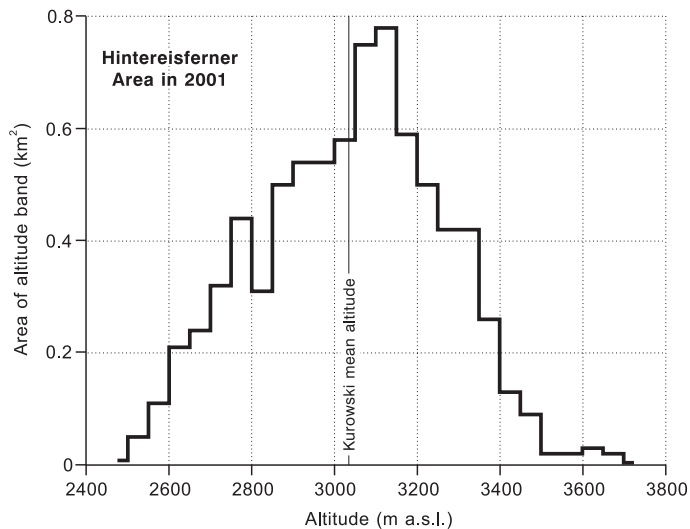
Figure 1. Area-altitude distribution for Hintereisferner, Austran Alps, showing areas of altitude bands vs. their mean altitudes. Area distribution is for year 2001.
