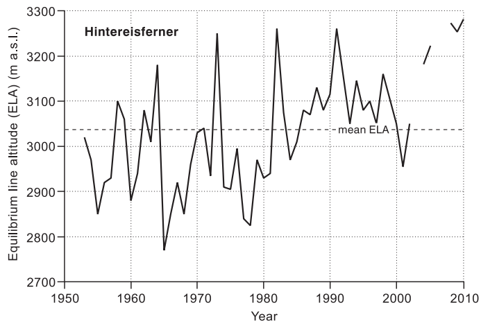
Figure 3. Year-to-year variations in equilibrium line altitude (ELA) at Hintereisferner, Austrian Alps, as measured in a surface mass balance programme for 1953–2010.
