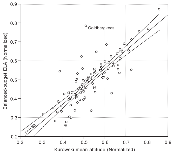
Figure 7. Balanced-budget ELA vs. Kurowski's mean altitude for 103 glaciers with both variables normalized to the altitude range of the glaciers. Normalized Y = (YH_{\min}) / (H_{\max} - H_{\min}) . Dashed lines denote 95 % confidence interval around the regression line according to Student t statistic (Kreyszig, 1970, p. 302).
