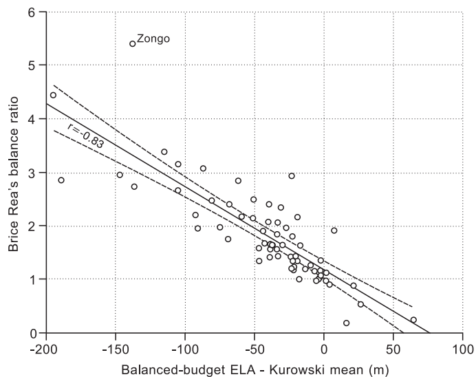
Figure 10. Brice Rea's balance ratio (Rea, 2009) plotted against Kurowski error ( ELA_0 - H_{\text{mean}} ) for 65 glaciers. Dashed lines denote 95 % confidence interval around the regression line according to Student t statistic (Kreyszig, 1970, p. 302).
