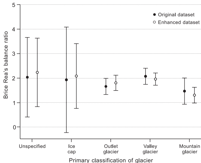
Figure 11. Brice Rea's balance ratio (Rea, 2009) vs. primary classification of glacier. Version 1 is for the original data (66 glaciers) and Version 2 is for an augmented data set (103 glaciers) using regression line in Fig. 10. Error bars represent 95 % confidence intervals of the means according to Student t statistic (Kreyszig, 1970, p. 178).
