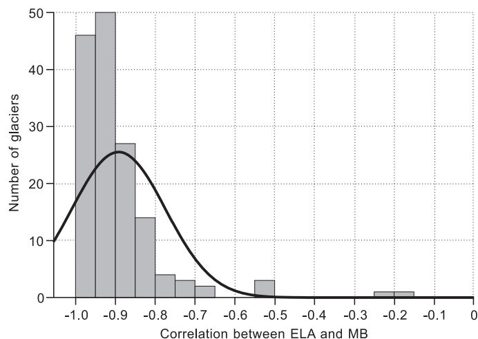
Figure 5. Histogram showing number of glaciers vs. correlation coefficients between equilibrium line altitude (ELA) and mean specific balance. Bold line denotes Gaussian curve with same mean and standard deviation.
