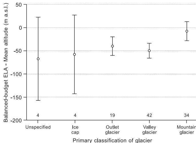
Figure 9. Boxplot of mean balanced-budget ELA minus Kurowski mean altitude ( ELA_0 - H_{\text{mean}} ) vs. primary classification of glaciers. Error bars represent 95 % confidence intervals of the means according to Student t statistic (Kreyszig, 1970, p. 178). Number of glaciers in each group are given in the lower part of the diagram.
