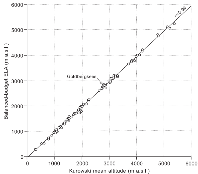
Figure 6. Balanced-budget ELA vs. Kurowski's mean altitude for 103 glaciers.
