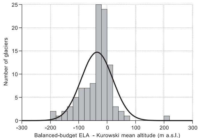
Figure 8. Histogram of difference between balanced-budget ELA and Kurowski mean altitude for 103 glaciers. Bold line denotes Gaussian curve with same mean and standard deviation.
