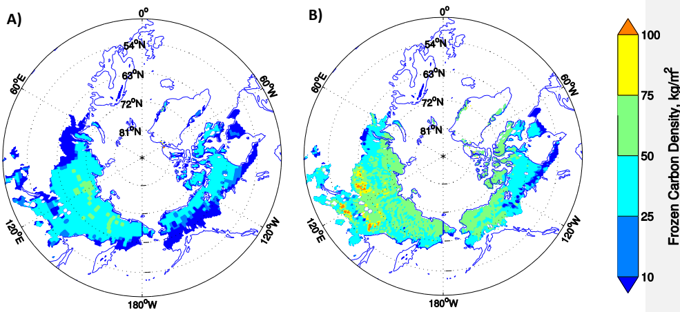
Figure 6. The frozen carbon maps obtained assuming uniform frozen carbon distribution at the initial time step, and averaged over five years at the end of the steady state run: A) from Schaefer et al., (2011), and B) from the current run, correspondingly.
