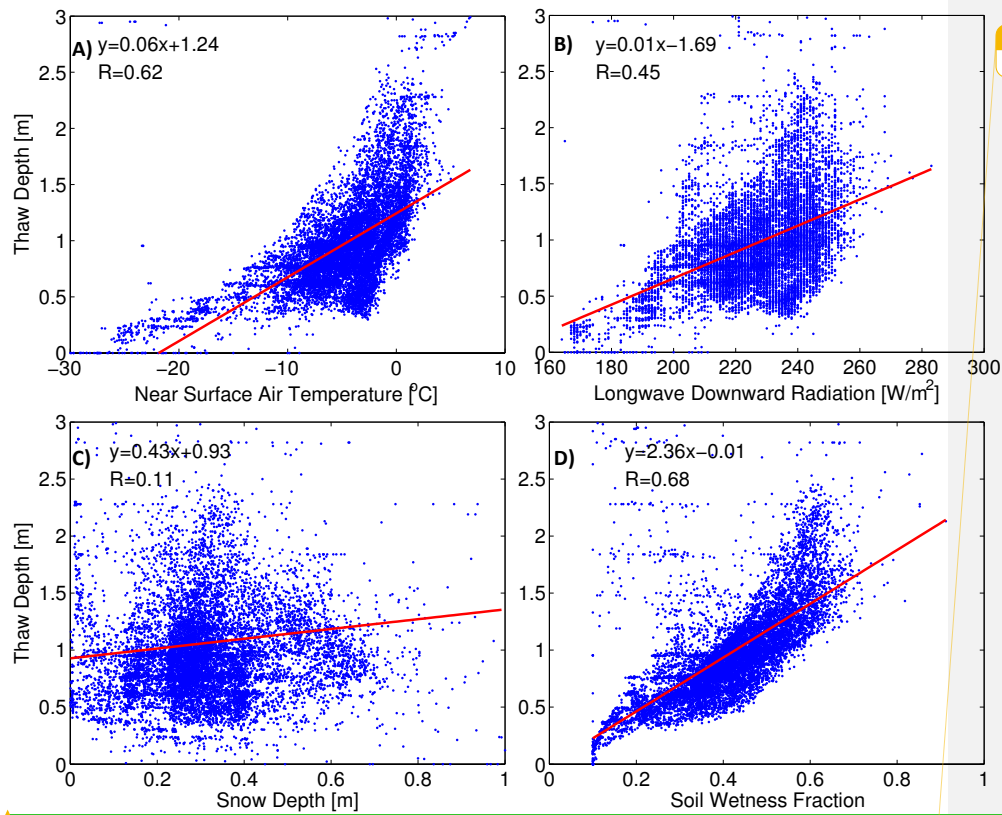
Figure 9. The correlation between ALT and: A) near air temperature for averaged over first two month of the fall season, and B) the down-welling long-wave radiation, averaged yearly over 10 years. C) the maximum snow depth over 10 years for the steady state run, and D) the soil wetness fraction, averaged yearly over 10 years.
