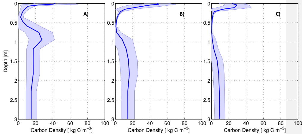
Figure 5. An averaged soil carbon distribution from 200 grid cells A) for the tundra region in continuous permafrost zone, B) for the boreal forest on the boundary between continuous and discontinuous zones, and C) for the low carbon soil at the south border of the discontinuous permafrost zone. The solid blue curve indicates the mean the white blue shading indicate the spread in the soil carbon density.
