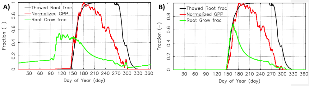
Figure 3: A) and B) root growth without and with the frozen soil constraint on growth.
