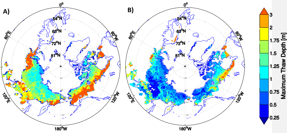
Figure 1. Maximum thaw depth averaged over last five years after spinup from A) Schaefer et al., (2011) and B) this study, in meters.
