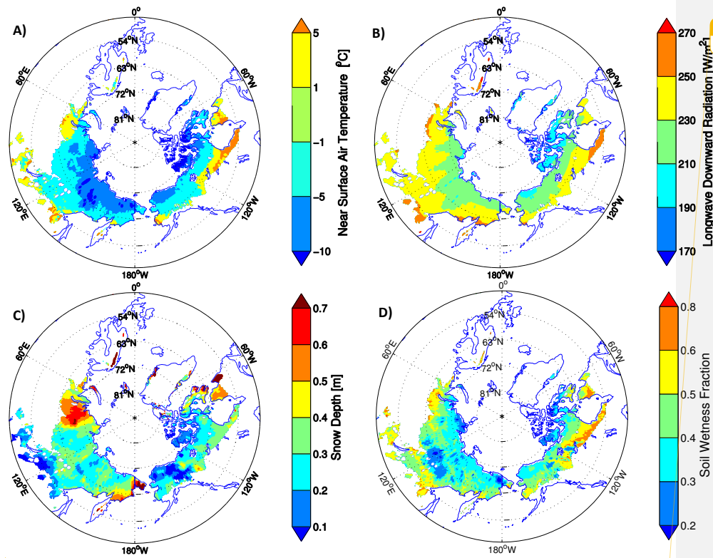
Figure 8. A) The near air temperature for averaged over first two month of the fall season. B) The down-welling long-wave radiation, averaged yearly over 10 years. C) The maximum snow depth obtained over 10 years for the steady state run, and D) the soil wetness fraction (dimensionless fraction of 1), representing overall near-surface soil wetness, averaged yearly over 10 years.
