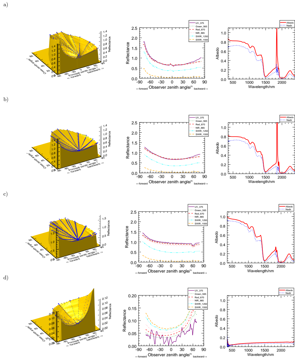
Figure 10. As in Fig. 9. Sooted snow on the 4 April 2013. (a) started at 9:56 with 68^\circ SZA; (b) 10:31, 62^\circ , (c) 11:18, 63^\circ , (d) natural snow sample at 13:31, 62^\circ .
