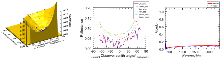
Figure 10. As in Fig. 9. Sooted snow on the 4 April 2013. (a) started at 9:56 with 68° SZA; (b) 10:31, 62°, (c) 11:18, 63°, (d) natural snow sample at 13:31, 62°.
