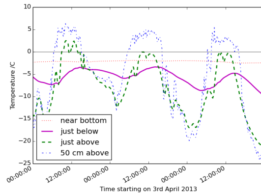
Figure 7. The snow and air temperatures measured by an FMI weather station at a swamp near Tähtelä, So-dankylä, few kilometers from the airport. The bottom value is measured at the interface between snow and ground, “just below” is 1–9cm below the snow surface, and “just above” 9–1cm above.
