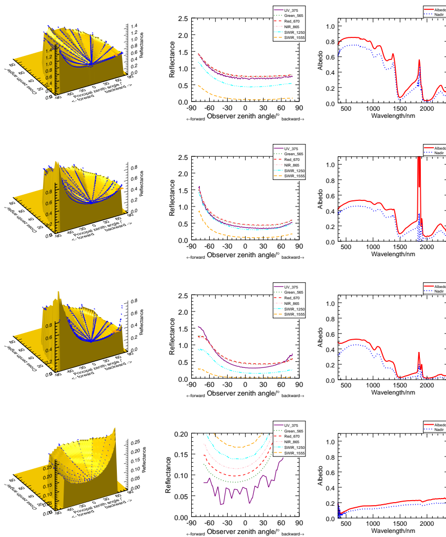
Figure 11. As in Fig. 9. (a) 10 g of silt /0.5 m 2 on top of snow, on the 4 April 2013 at 15:05, 65°, (b) 10 g of silt/0.5 m 2 , on the 4 April 2013 at 16:29, 72°, note large SZA, (c) same sample on the 5 April 2013 at 11:16, 61°, most difference to b due to different SZA, (d) pure silt measured in laboratory, 65°.
