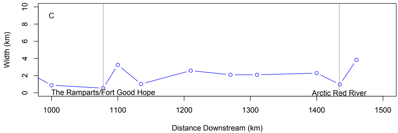
Figure 7: Change in channel width along the Mackenzie River as observed in A (ca. 0-500 km), B (ca. 500-1000 km) and C (ca. 1000-1500 km).
